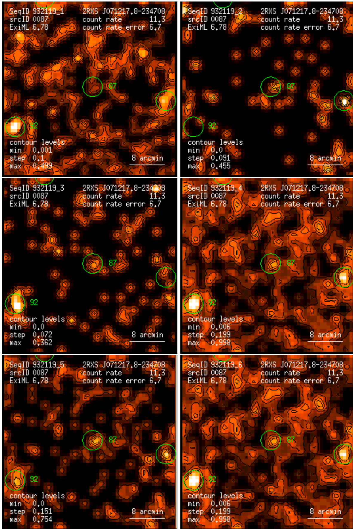
Figure 87: RASS 932119: detection 0087: band rate images, Gaussian filter: (1) PSPC channels 11 – 41, (2) 52 – 90, (3) 91 – 201, (4) 11 – 235, (5) 52 – 201, (6) 11 – 201. Broad band rates in counts/ks. Band rate contour levels in counts/ks/arcmin 2 .
