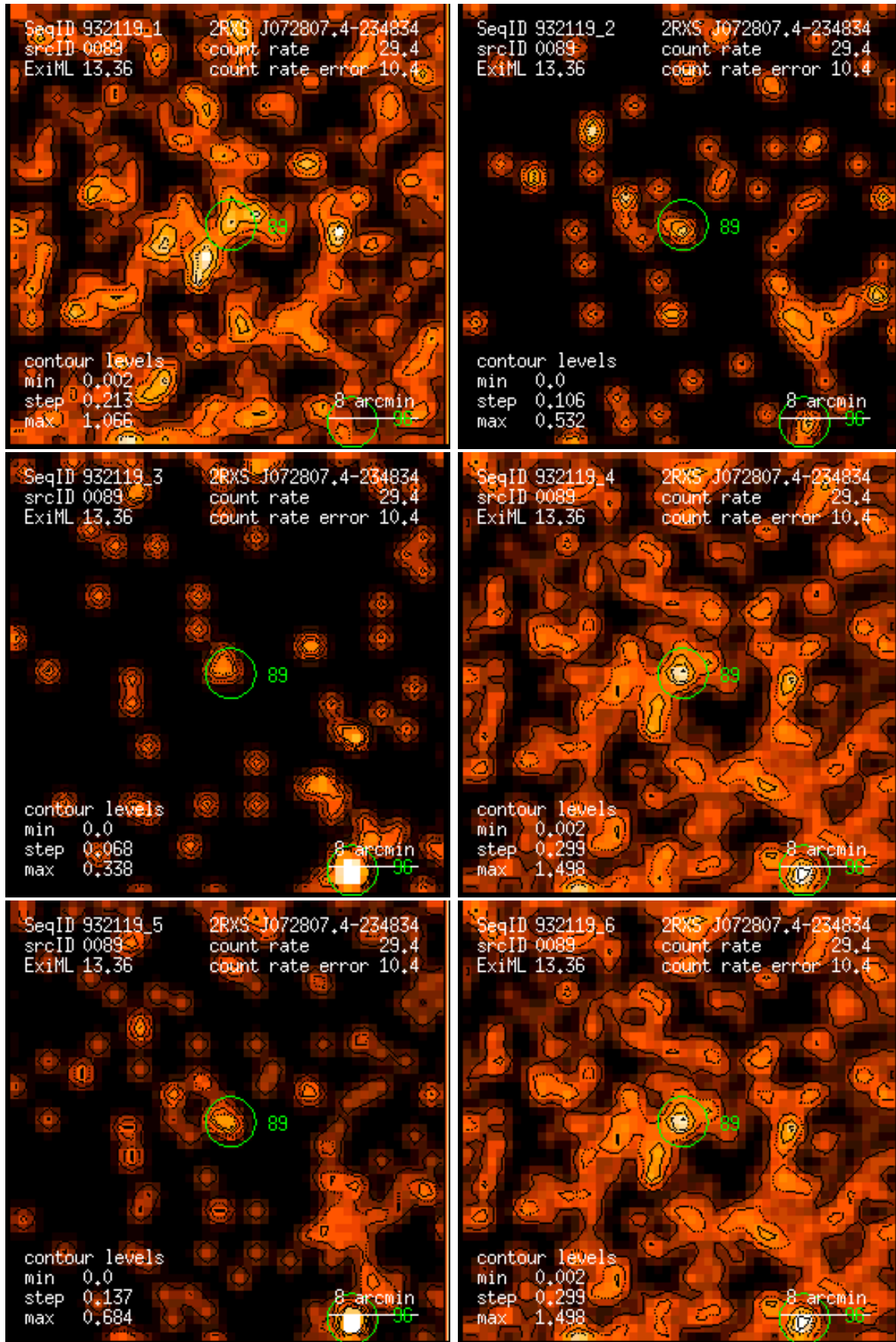
Figure 89: RASS 932119: detection 0089: band rate images, Gaussian filter: (1) PSPC channels 11 – 41, (2) 52 – 90, (3) 91 – 201, (4) 11 – 235, (5) 52 – 201, (6) 11 – 201. Broad band rates in counts/ks. Band rate contour levels in counts/ks/arcmin 2 .
