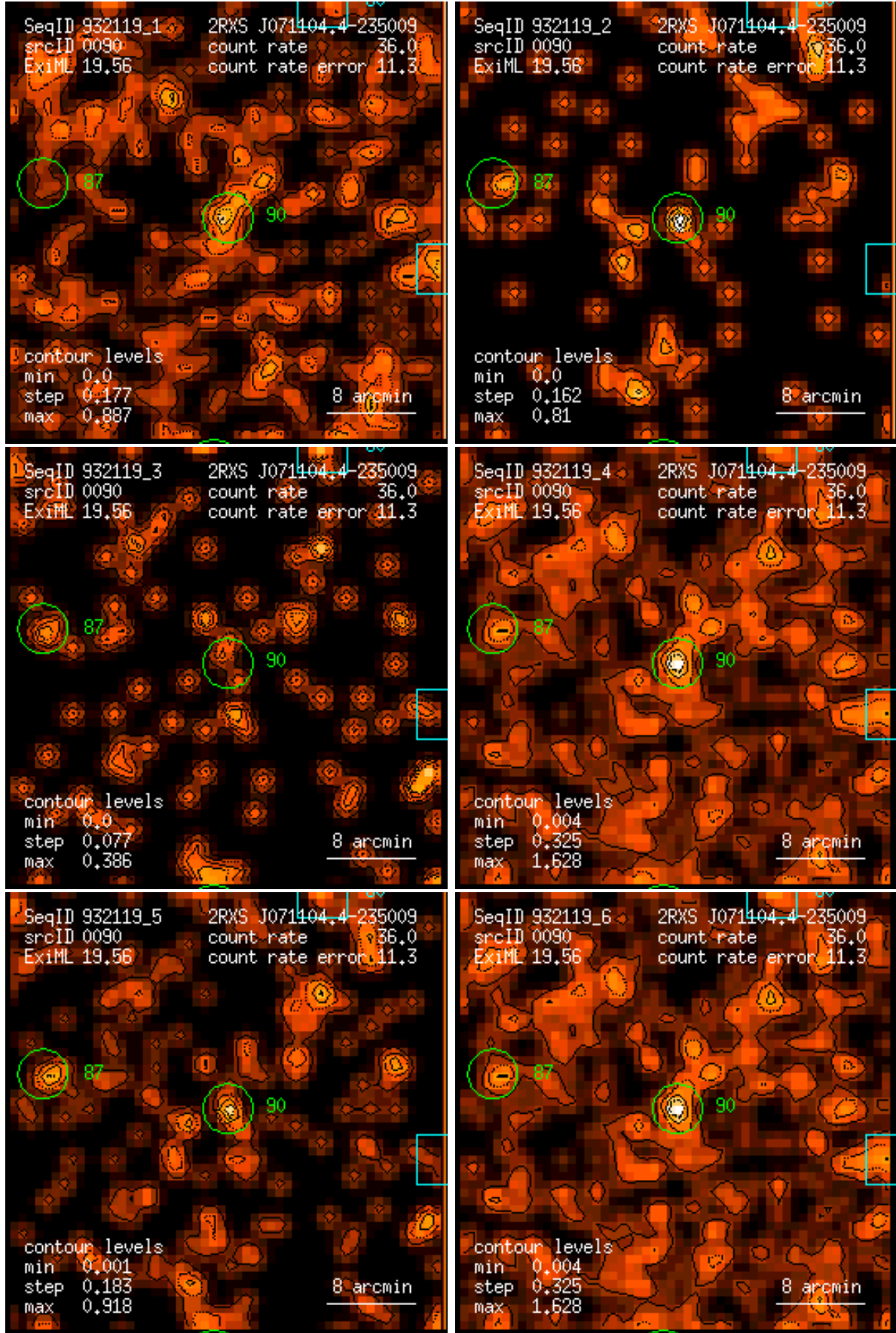
Figure 90: RASS 932119: detection 0090: band rate images, Gaussian filter: (1) PSPC channels 11 – 41, (2) 52 – 90, (3) 91 – 201, (4) 11 – 235, (5) 52 – 201, (6) 11 – 201. Broad band rates in counts/ks. Band rate contour levels in counts/ks/arcmin 2 .
