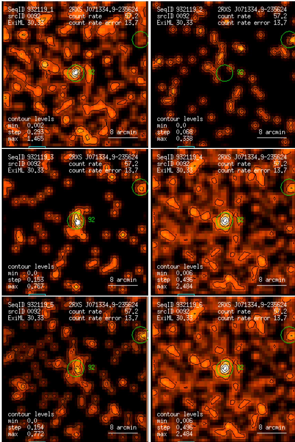
Figure 92: RASS 932119: detection 0092: band rate images, Gaussian filter: (1) PSPC channels 11 – 41, (2) 52 – 90, (3) 91 – 201, (4) 11 – 235, (5) 52 – 201, (6) 11 – 201. Broad band rates in counts/ks. Band rate contour levels in counts/ks/arcmin 2 .
