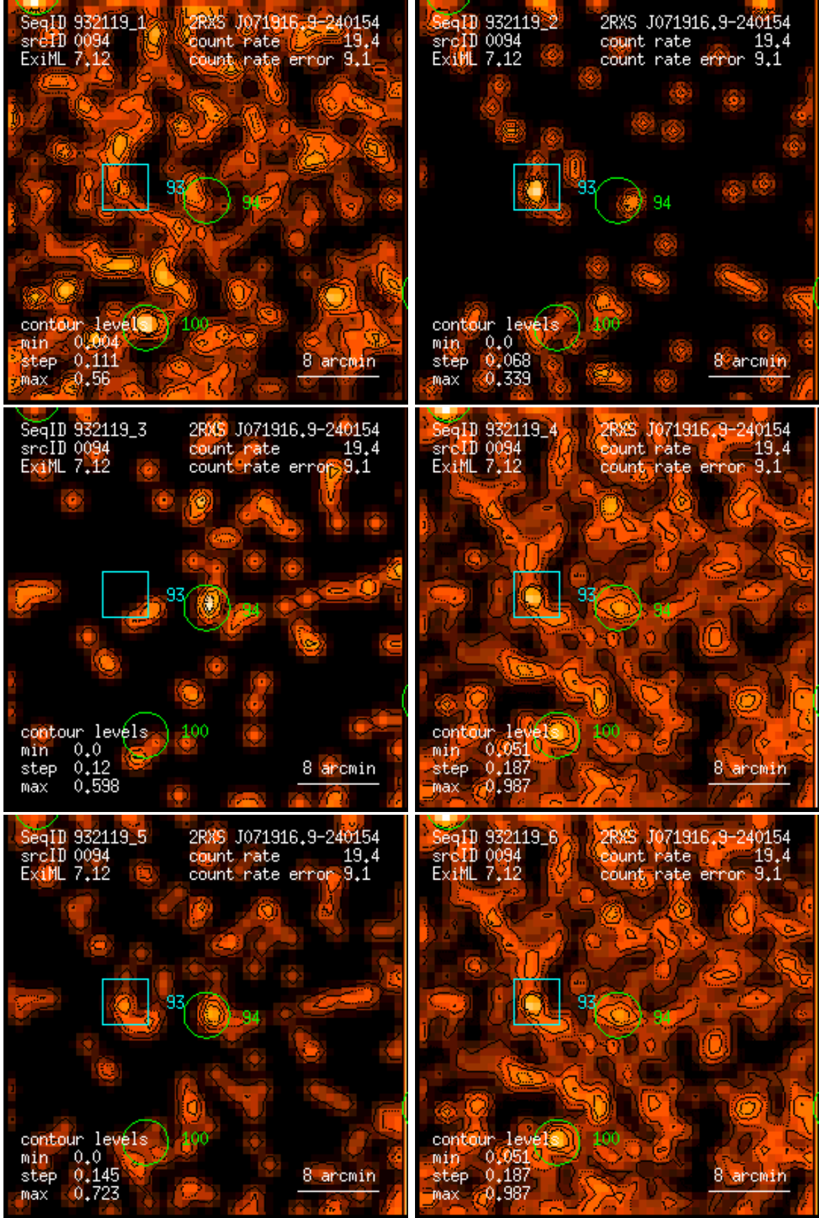
Figure 94: RASS 932119: detection 0094: band rate images, Gaussian filter: (1) PSPC channels 11 – 41, (2) 52 – 90, (3) 91 – 201, (4) 11 – 235, (5) 52 – 201, (6) 11 – 201. Broad band rates in counts/ks. Band rate contour levels in counts/ks/arcmin 2 .
