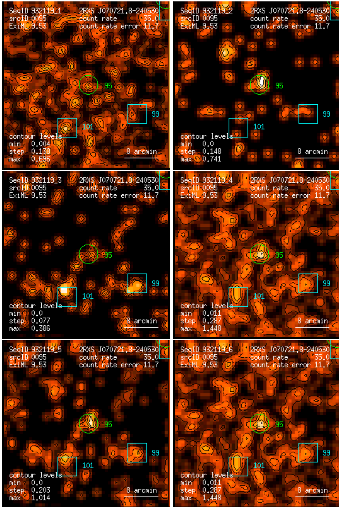
Figure 95: RASS 932119: detection 0095: band rate images, Gaussian filter: (1) PSPC channels 11 – 41, (2) 52 – 90, (3) 91 – 201, (4) 11 – 235, (5) 52 – 201, (6) 11 – 201. Broad band rates in counts/ks. Band rate contour levels in counts/ks/arcmin 2 .
