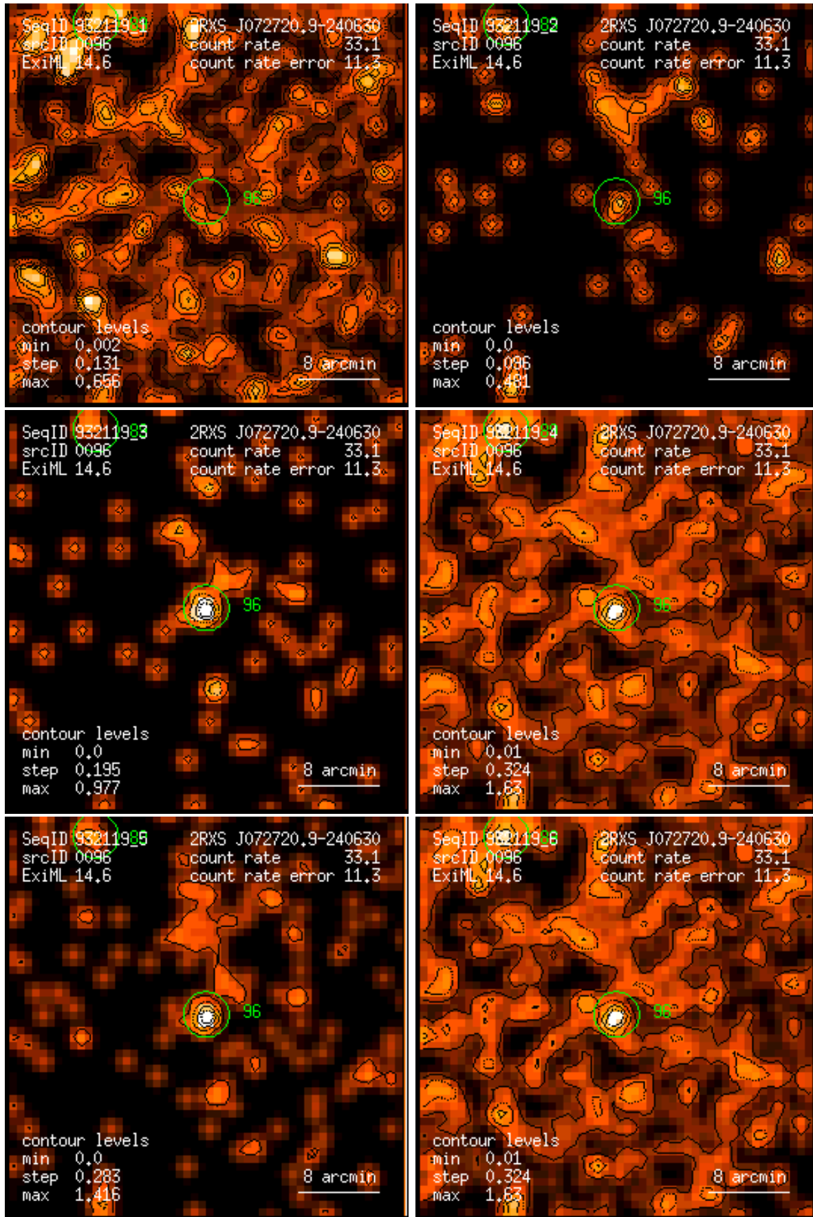
Figure 96: RASS 932119: detection 0096: band rate images, Gaussian filter: (1) PSPC channels 11 – 41, (2) 52 – 90, (3) 91 – 201, (4) 11 – 235, (5) 52 – 201, (6) 11 – 201. Broad band rates in counts/ks. Band rate contour levels in counts/ks/arcmin 2 .
