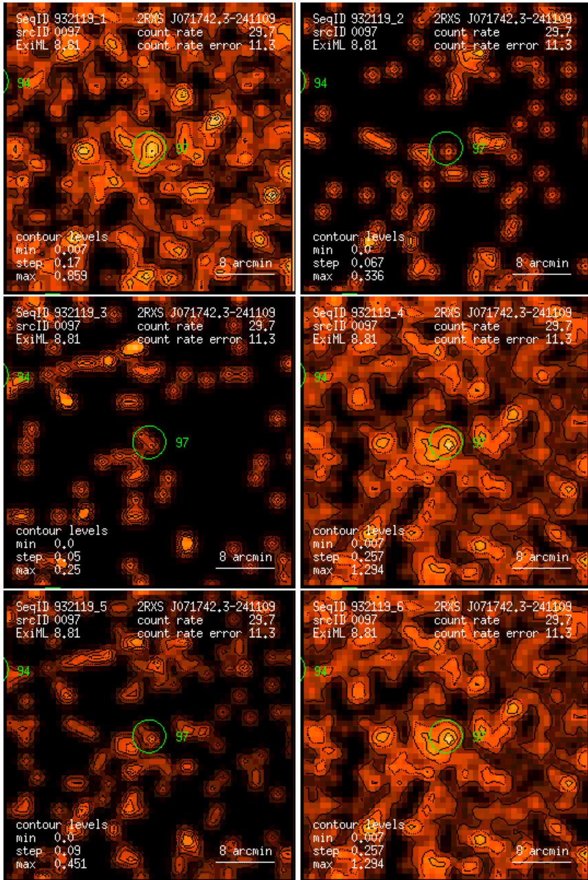
Figure 97: RASS 932119: detection 0097: band rate images, Gaussian filter: (1) PSPC channels 11 – 41, (2) 52 – 90, (3) 91 – 201, (4) 11 – 235, (5) 52 – 201, (6) 11 – 201. Broad band rates in counts/ks. Band rate contour levels in counts/ks/arcmin 2 .
