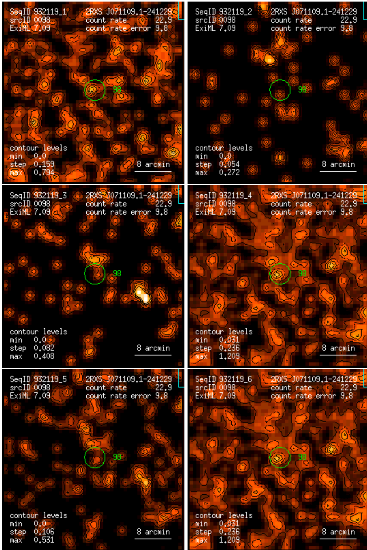
Figure 98: RASS 932119: detection 0098: band rate images, Gaussian filter: (1) PSPC channels 11 – 41, (2) 52 – 90, (3) 91 – 201, (4) 11 – 235, (5) 52 – 201, (6) 11 – 201. Broad band rates in counts/ks. Band rate contour levels in counts/ks/arcmin 2 .
