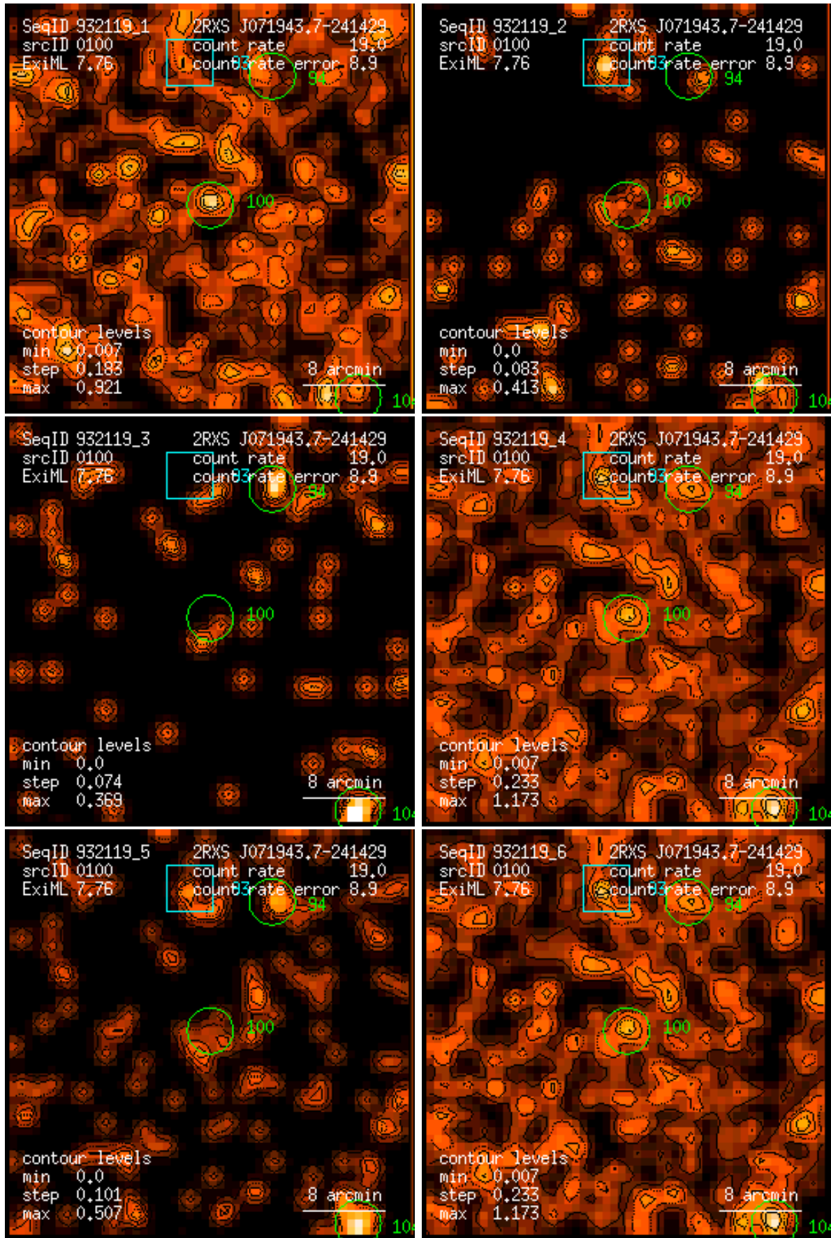
Figure 100: RASS 932119: detection 0100: band rate images, Gaussian filter: (1) PSPC channels 11 – 41, (2) 52 – 90, (3) 91 – 201, (4) 11 – 235, (5) 52 – 201, (6) 11 – 201. Broad band rates in counts/ks. Band rate contour levels in counts/ks/arcmin 2 .
