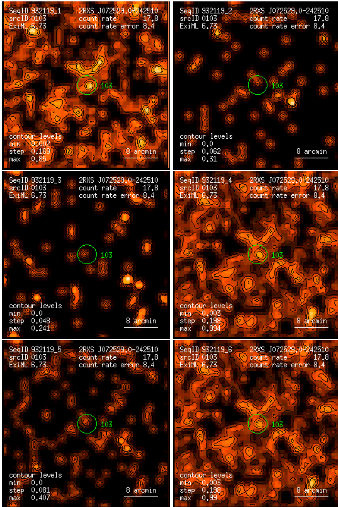
Figure 103: RASS 932119: detection 0103: band rate images, Gaussian filter: (1) PSPC channels 11 – 41, (2) 52 – 90, (3) 91 – 201, (4) 11 – 235, (5) 52 – 201, (6) 11 – 201. Broad band rates in counts/ks. Band rate contour levels in counts/ks/arcmin 2 .
