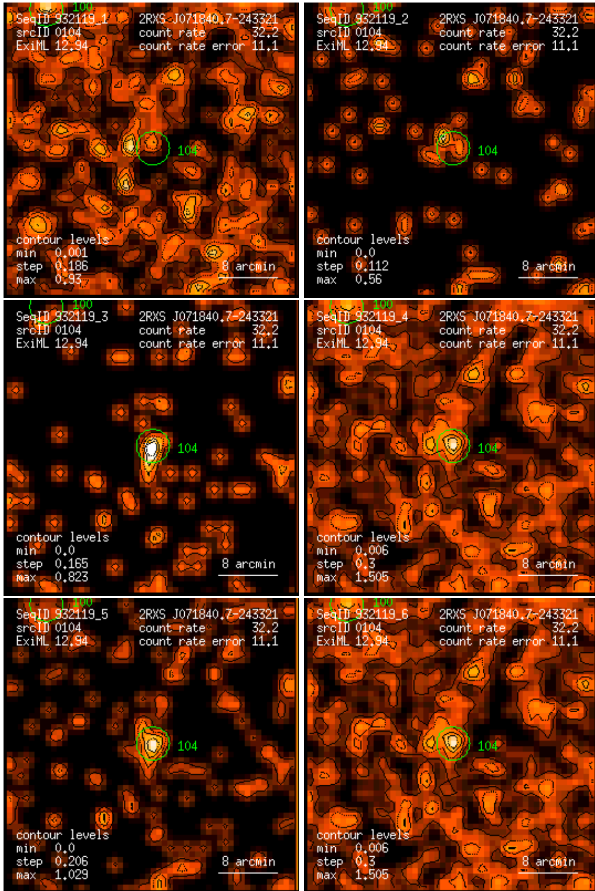
Figure 104: RASS 932119: detection 0104: band rate images, Gaussian filter: (1) PSPC channels 11 – 41, (2) 52 – 90, (3) 91 – 201, (4) 11 – 235, (5) 52 – 201, (6) 11 – 201. Broad band rates in counts/ks. Band rate contour levels in counts/ks/arcmin 2 .
