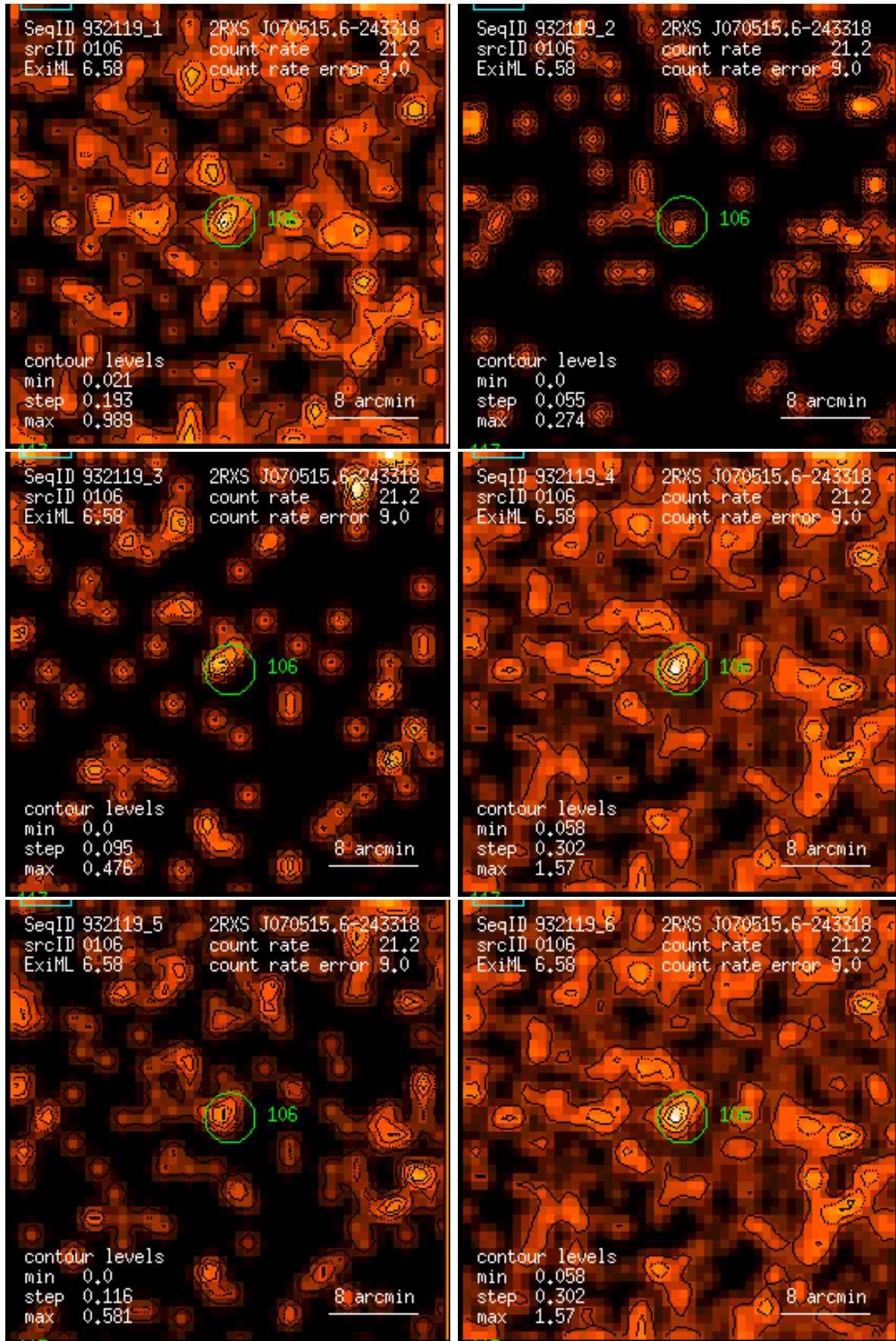
Figure 106: RASS 932119: detection 0106: band rate images, Gaussian filter: (1) PSPC channels 11 – 41, (2) 52 – 90, (3) 91 – 201, (4) 11 – 235, (5) 52 – 201, (6) 11 – 201. Broad band rates in counts/ks. Band rate contour levels in counts/ks/arcmin 2 .
