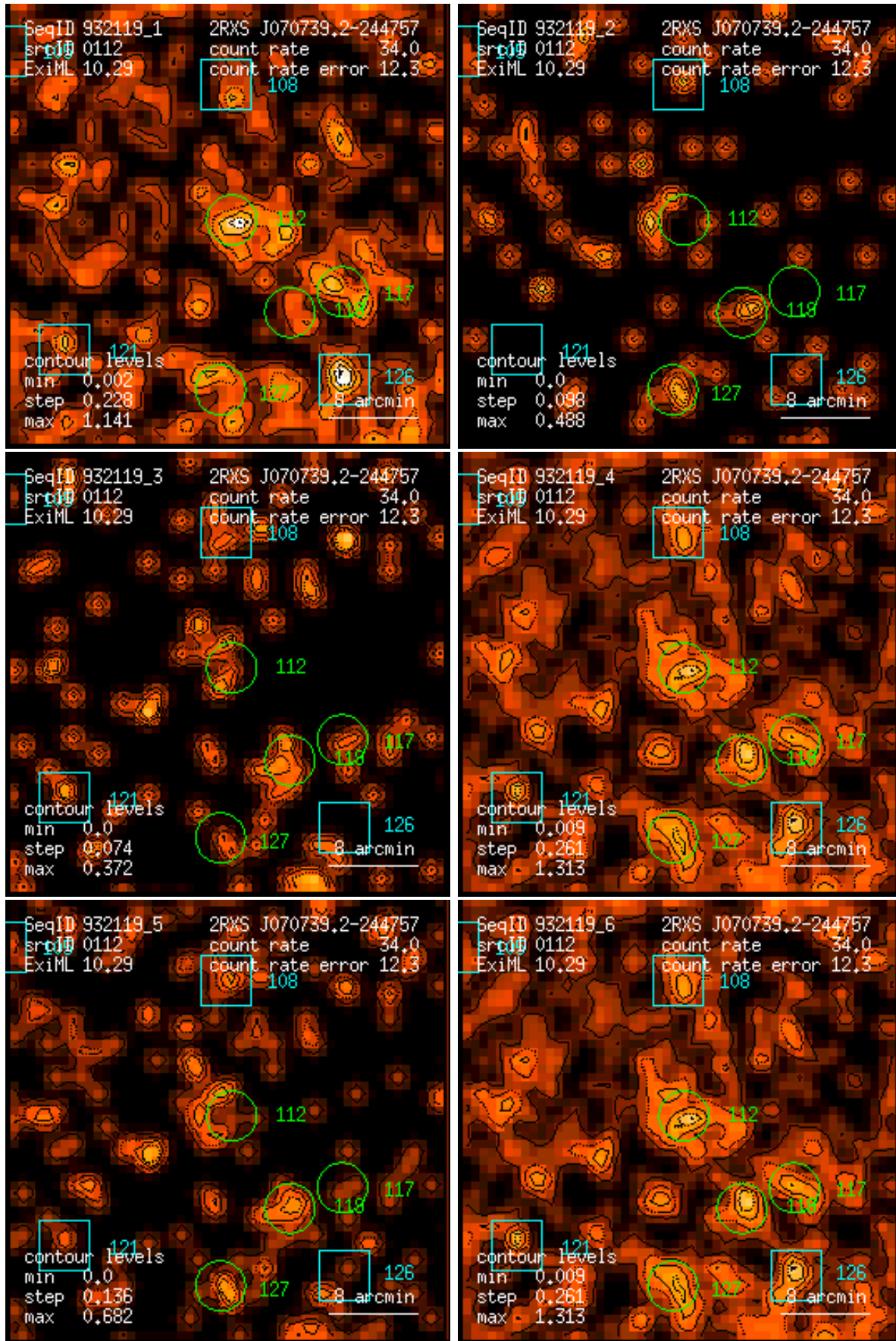
Figure 112: RASS 932119: detection 0112: band rate images, Gaussian filter: (1) PSPC channels 11 – 41, (2) 52 – 90, (3) 91 – 201, (4) 11 – 235, (5) 52 – 201, (6) 11 – 201. Broad band rates in counts/ks. Band rate contour levels in counts/ks/arcmin 2 .
