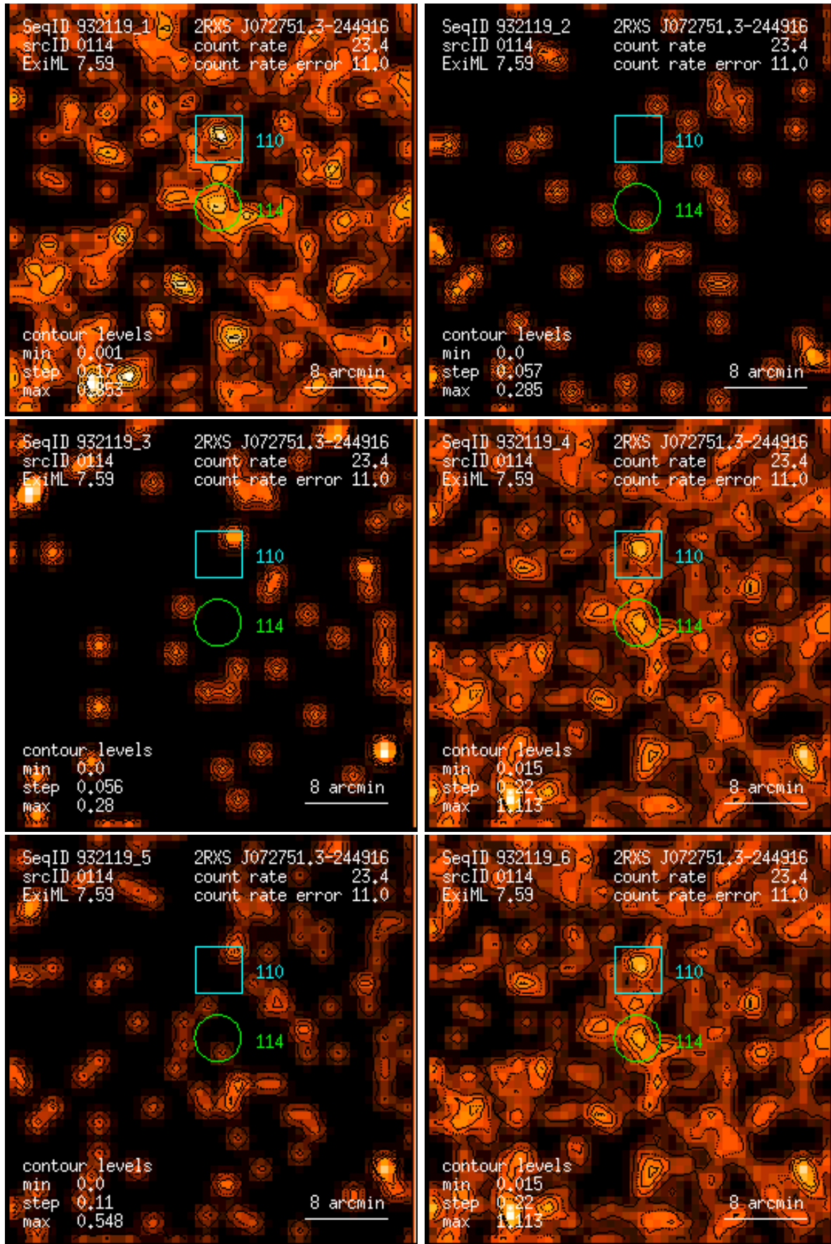
Figure 114: RASS 932119: detection 0114: band rate images, Gaussian filter: (1) PSPC channels 11 – 41, (2) 52 – 90, (3) 91 – 201, (4) 11 – 235, (5) 52 – 201, (6) 11 – 201. Broad band rates in counts/ks. Band rate contour levels in counts/ks/arcmin 2 .
