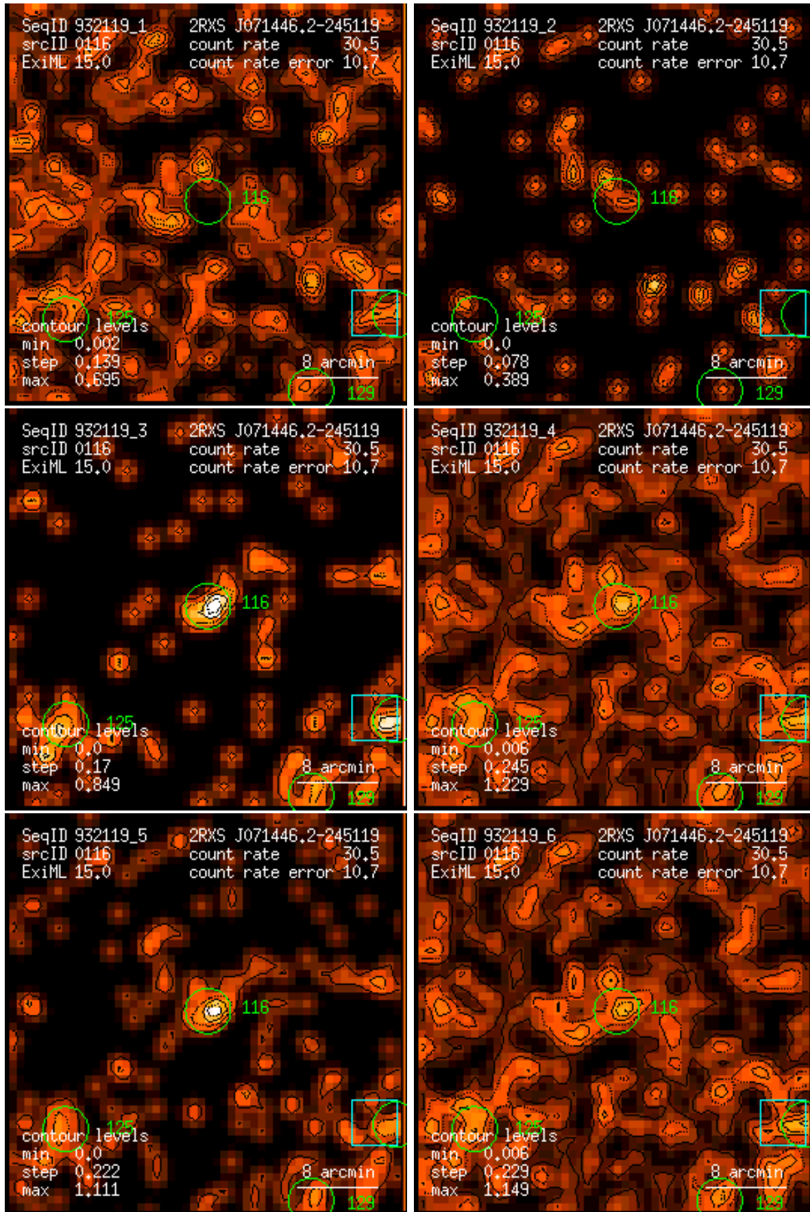
Figure 116: RASS 932119: detection 0116: band rate images, Gaussian filter: (1) PSPC channels 11 – 41, (2) 52 – 90, (3) 91 – 201, (4) 11 – 235, (5) 52 – 201, (6) 11 – 201. Broad band rates in counts/ks. Band rate contour levels in counts/ks/arcmin 2 .
