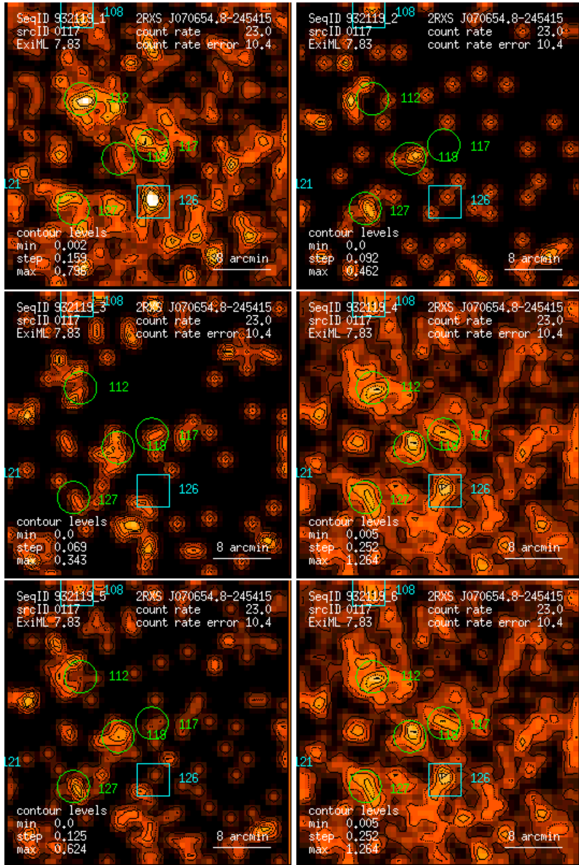
Figure 117: RASS 932119: detection 0117: band rate images, Gaussian filter: (1) PSPC channels 11 – 41, (2) 52 – 90, (3) 91 – 201, (4) 11 – 235, (5) 52 – 201, (6) 11 – 201. Broad band rates in counts/ks. Band rate contour levels in counts/ks/arcmin 2 .
