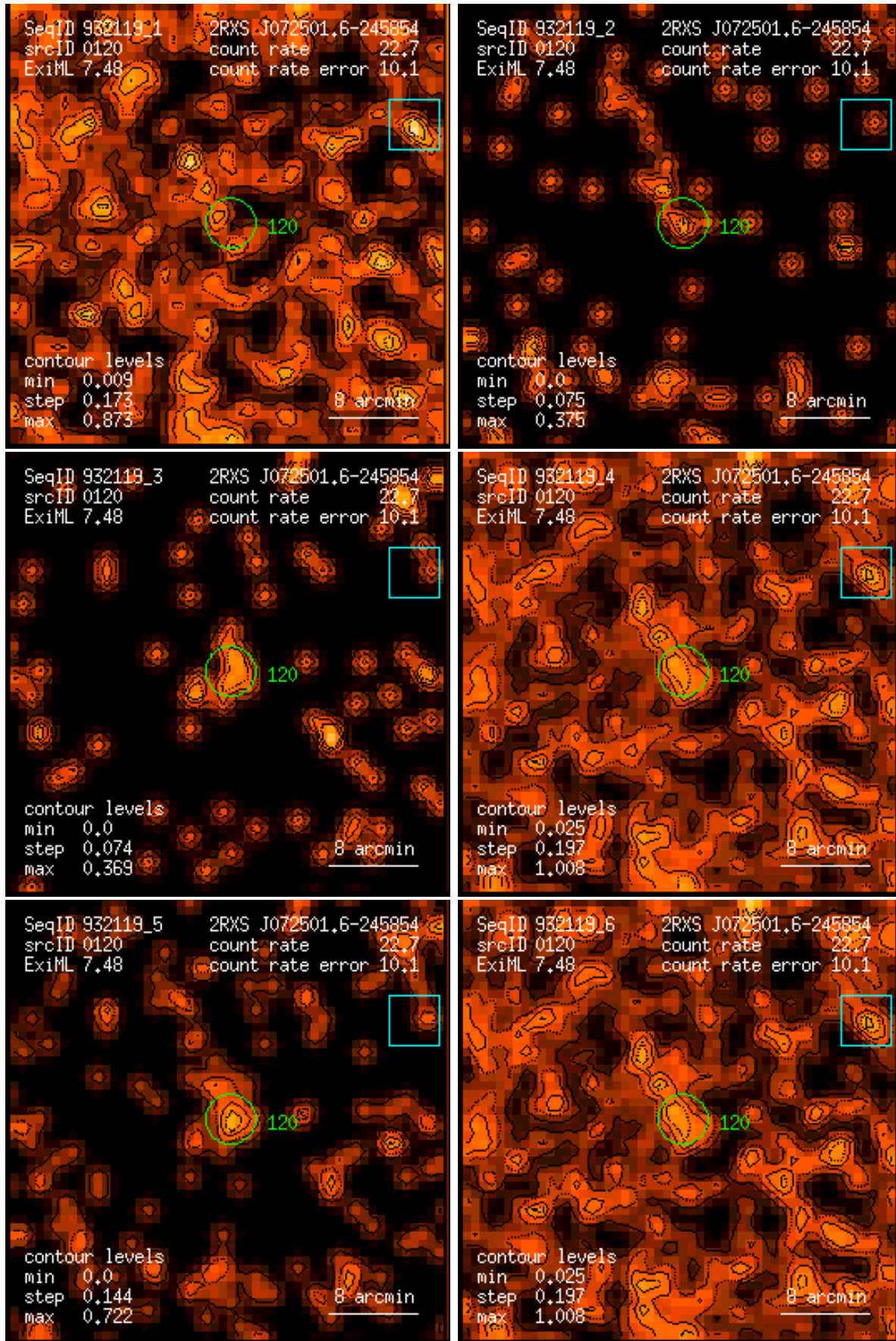
Figure 120: RASS 932119: detection 0120: band rate images, Gaussian filter: (1) PSPC channels 11 – 41, (2) 52 – 90, (3) 91 – 201, (4) 11 – 235, (5) 52 – 201, (6) 11 – 201. Broad band rates in counts/ks. Band rate contour levels in counts/ks/arcmin 2 .
