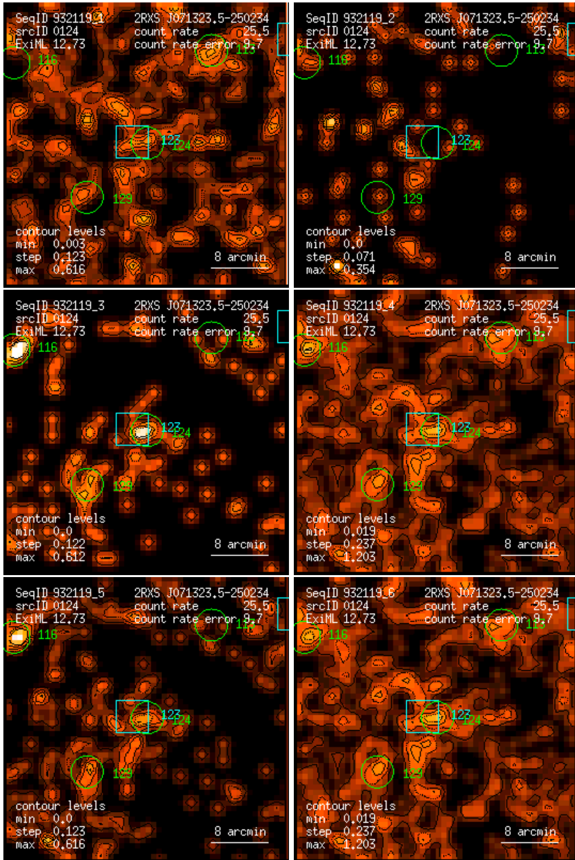
Figure 124: RASS 932119: detection 0124: band rate images, Gaussian filter: (1) PSPC channels 11 – 41, (2) 52 – 90, (3) 91 – 201, (4) 11 – 235, (5) 52 – 201, (6) 11 – 201. Broad band rates in counts/ks. Band rate contour levels in counts/ks/arcmin 2 .
