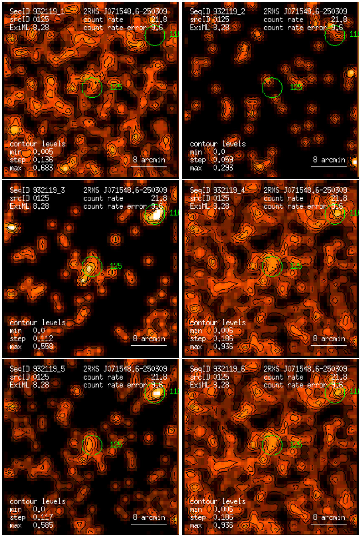
Figure 125: RASS 932119: detection 0125: band rate images, Gaussian filter: (1) PSPC channels 11 – 41, (2) 52 – 90, (3) 91 – 201, (4) 11 – 235, (5) 52 – 201, (6) 11 – 201. Broad band rates in counts/ks. Band rate contour levels in counts/ks/arcmin 2 .
