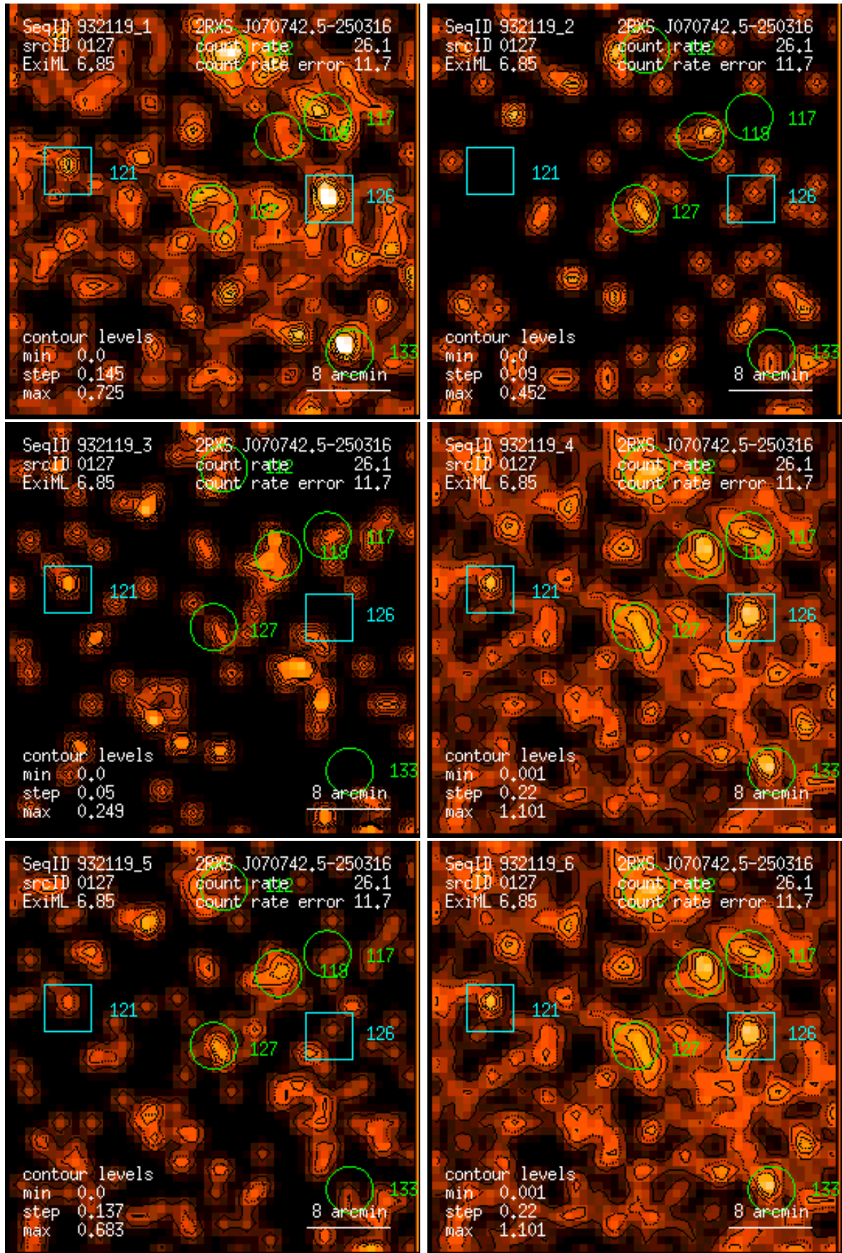
Figure 127: RASS 932119: detection 0127: band rate images, Gaussian filter: (1) PSPC channels 11 – 41, (2) 52 – 90, (3) 91 – 201, (4) 11 – 235, (5) 52 – 201, (6) 11 – 201. Broad band rates in counts/ks. Band rate contour levels in counts/ks/arcmin 2 .
