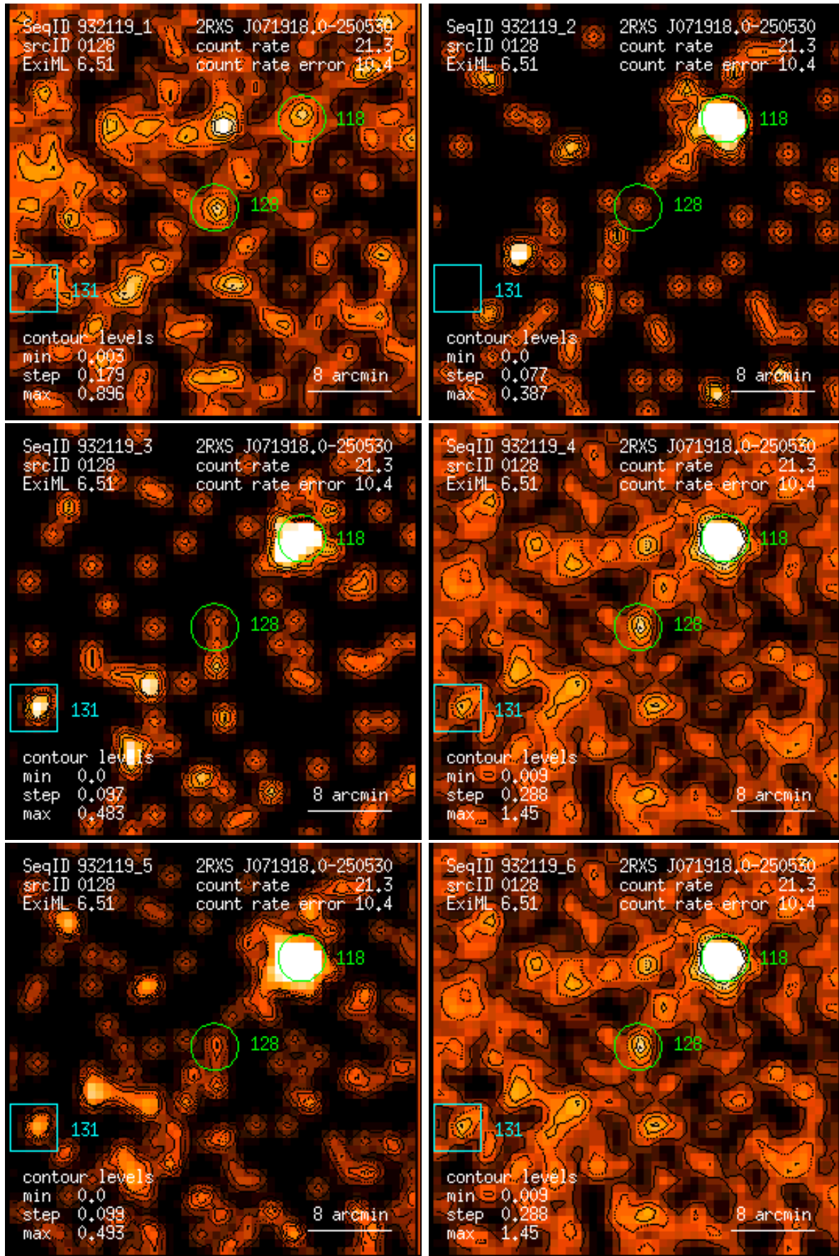
Figure 128: RASS 932119: detection 0128: band rate images, Gaussian filter: (1) PSPC channels 11 – 41, (2) 52 – 90, (3) 91 – 201, (4) 11 – 235, (5) 52 – 201, (6) 11 – 201. Broad band rates in counts/ks. Band rate contour levels in counts/ks/arcmin 2 .
