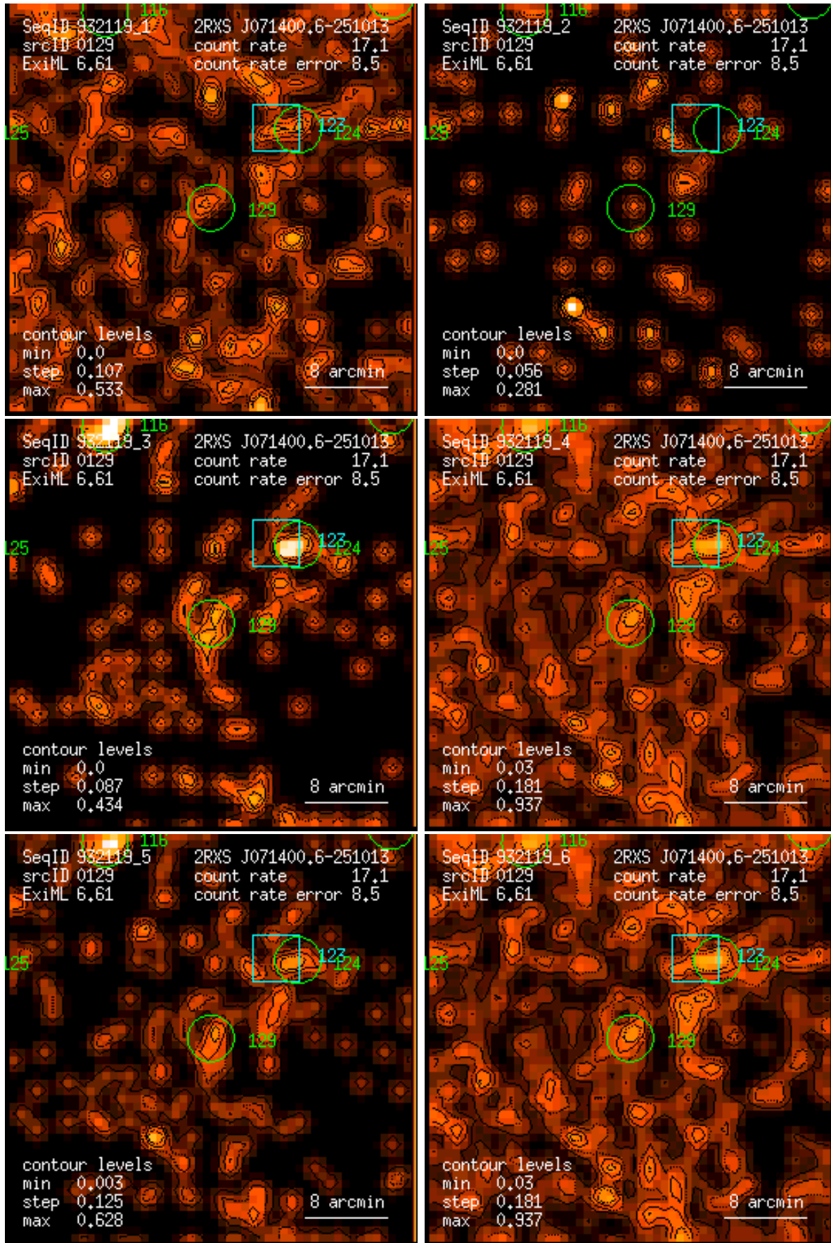
Figure 129: RASS 932119: detection 0129: band rate images, Gaussian filter: (1) PSPC channels 11 – 41, (2) 52 – 90, (3) 91 – 201, (4) 11 – 235, (5) 52 – 201, (6) 11 – 201. Broad band rates in counts/ks. Band rate contour levels in counts/ks/arcmin 2 .
