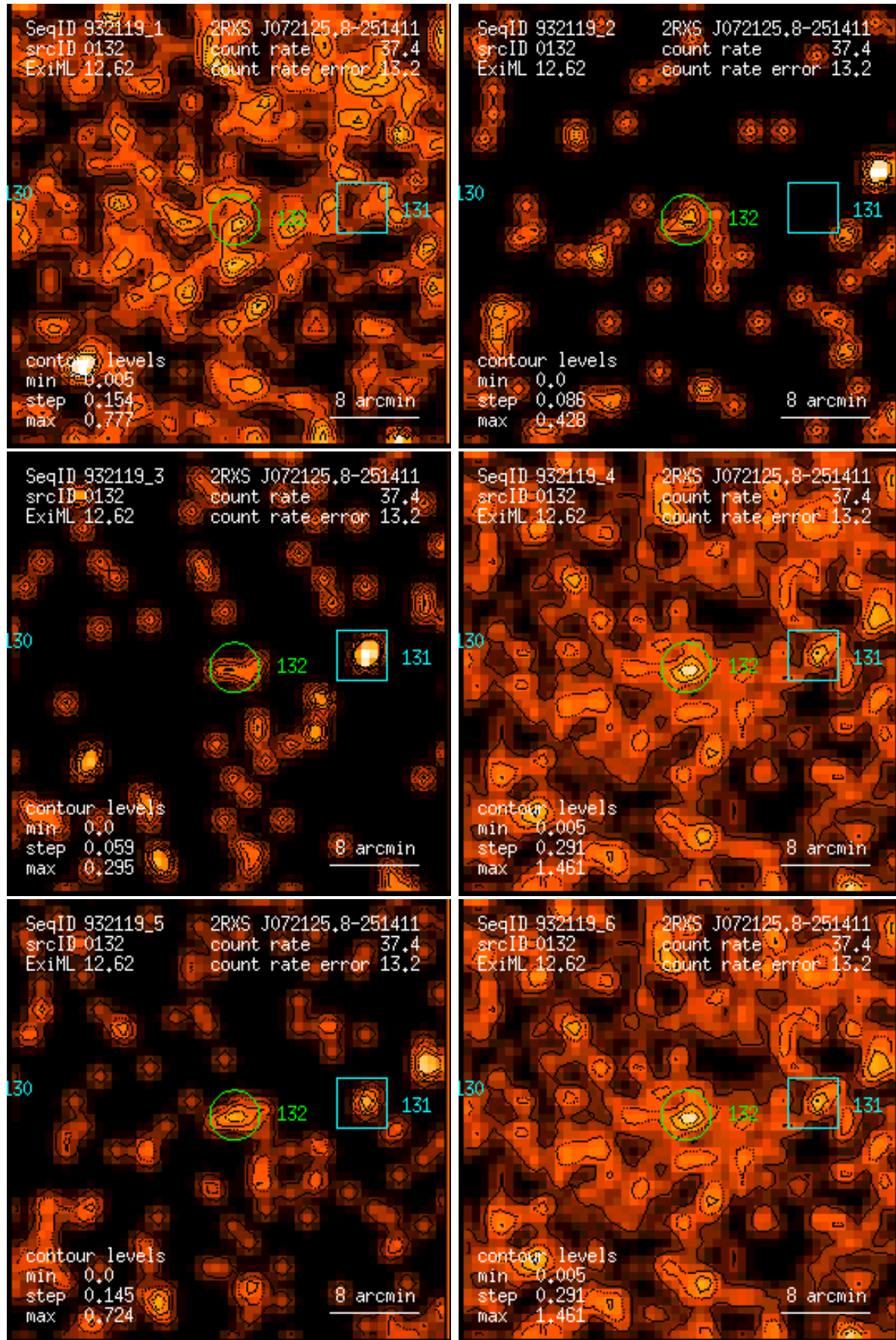
Figure 132: RASS 932119: detection 0132: band rate images, Gaussian filter: (1) PSPC channels 11 – 41, (2) 52 – 90, (3) 91 – 201, (4) 11 – 235, (5) 52 – 201, (6) 11 – 201. Broad band rates in counts/ks. Band rate contour levels in counts/ks/arcmin 2 .
