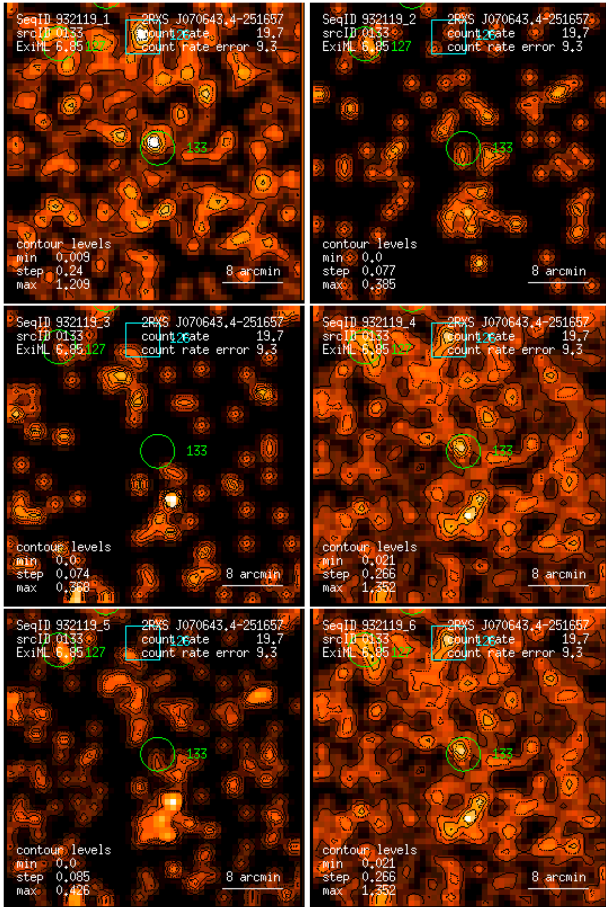
Figure 133: RASS 932119: detection 0133: band rate images, Gaussian filter: (1) PSPC channels 11 – 41, (2) 52 – 90, (3) 91 – 201, (4) 11 – 235, (5) 52 – 201, (6) 11 – 201. Broad band rates in counts/ks. Band rate contour levels in counts/ks/arcmin 2 .
