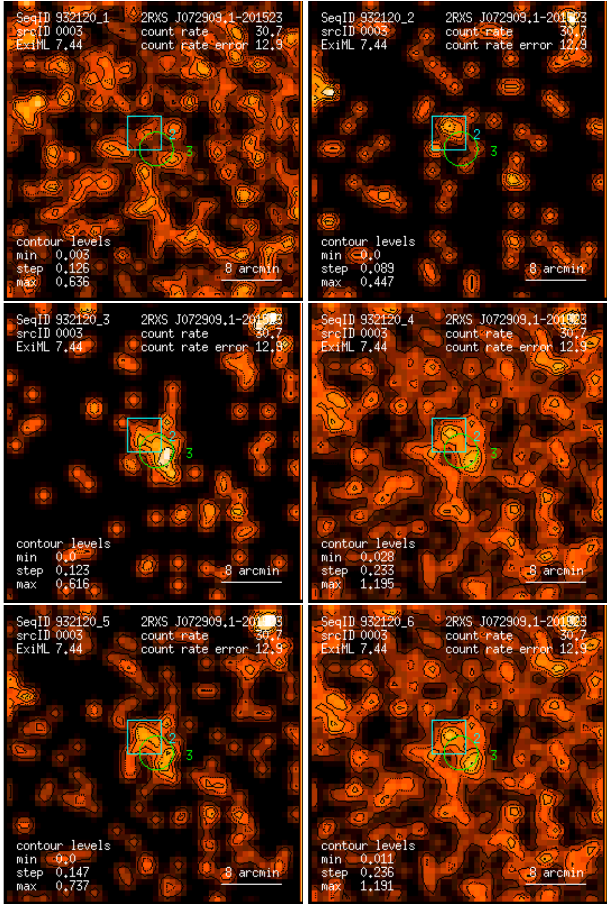
Figure 3: RASS 932120: detection 0003: band rate images, Gaussian filter: (1) PSPC channels 11 – 41, (2) 52 – 90, (3) 91 – 201, (4) 11 – 235, (5) 52 – 201, (6) 11 – 201. Broad band rates in counts/ks. Band rate contour levels in counts/ks/arcmin 2 .
