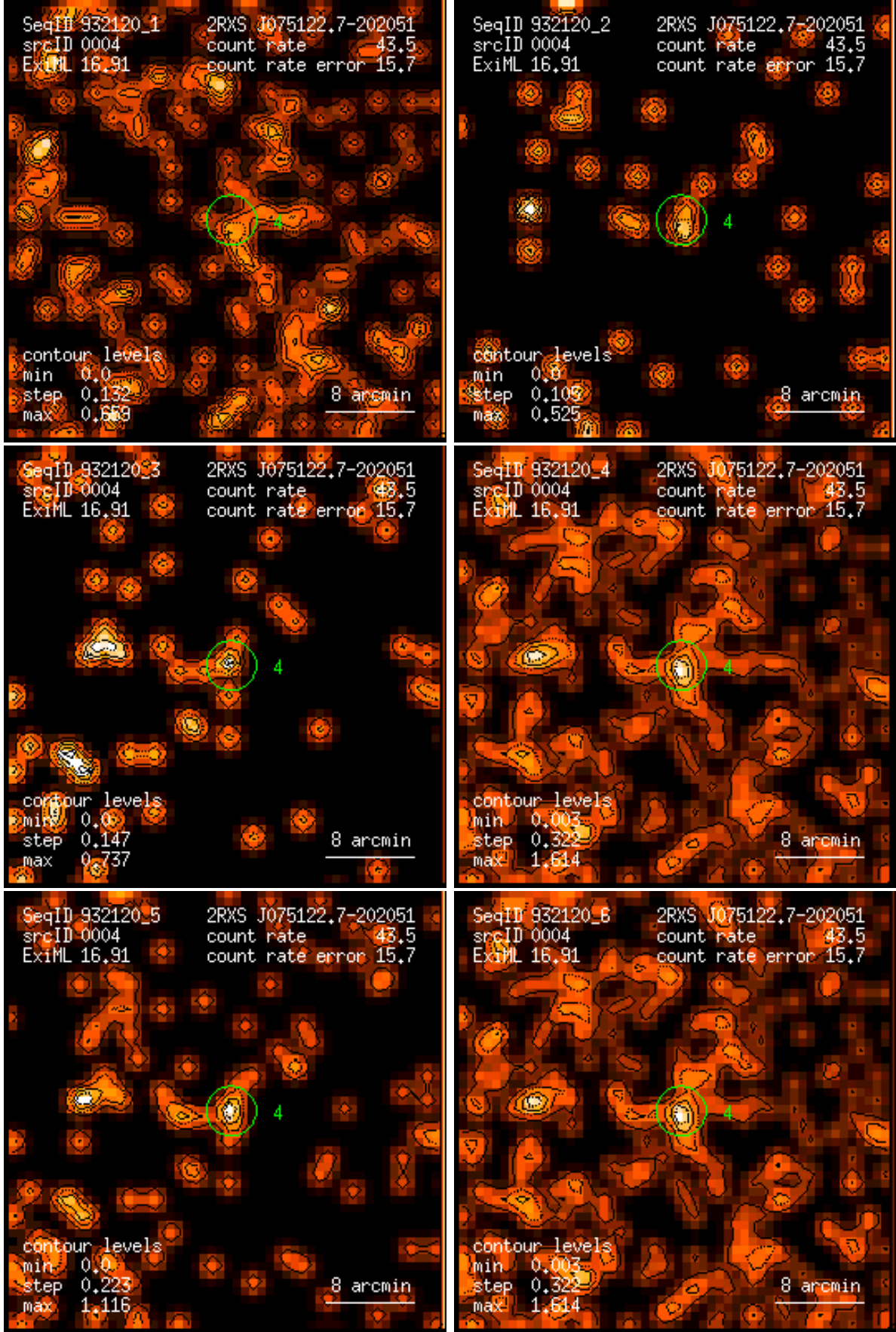
Figure 4: RASS 932120: detection 0004: band rate images, Gaussian filter: (1) PSPC channels 11 – 41, (2) 52 – 90, (3) 91 – 201, (4) 11 – 235, (5) 52 – 201, (6) 11 – 201. Broad band rates in counts/ks. Band rate contour levels in counts/ks/arcmin 2 .
