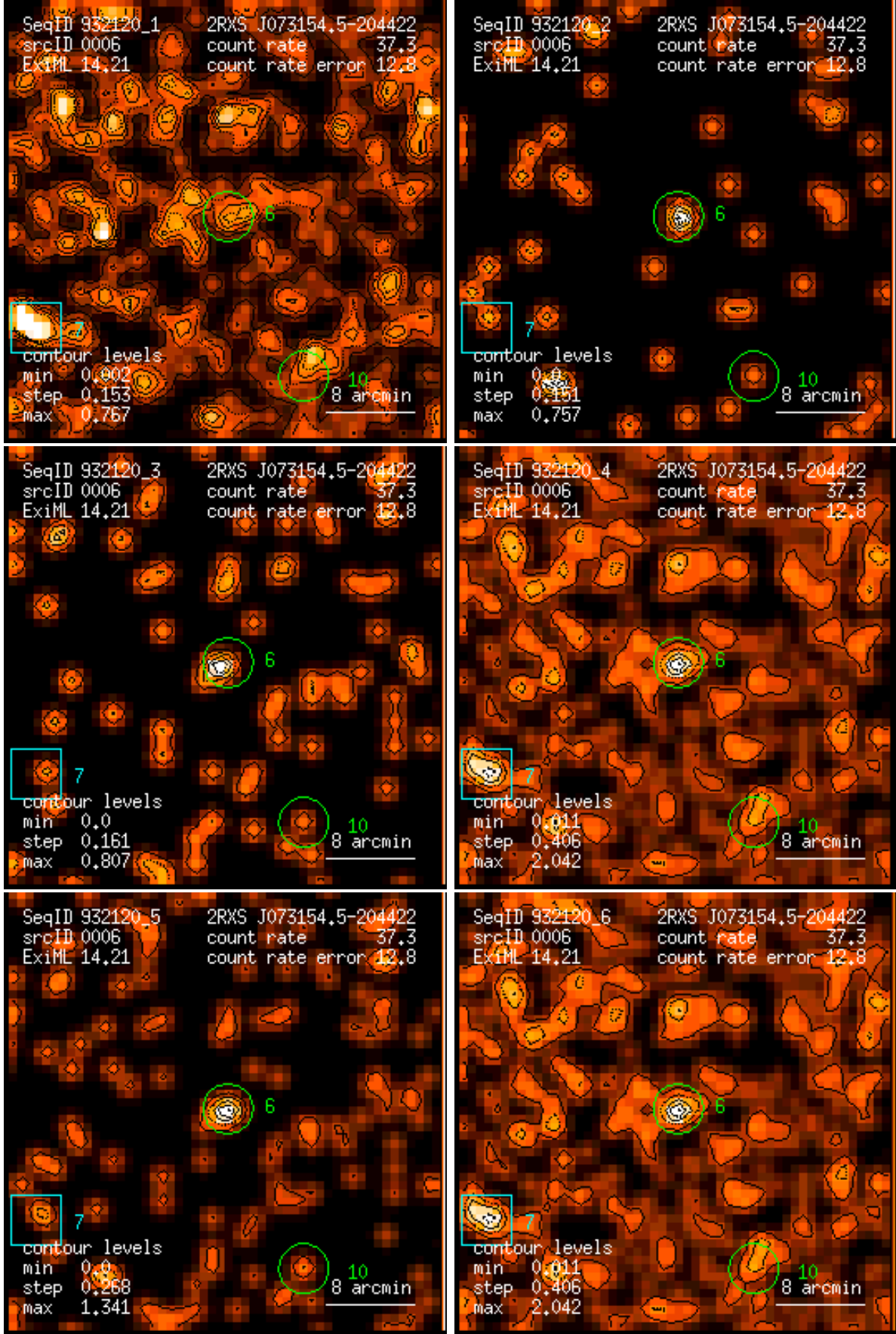
Figure 6: RASS 932120: detection 0006: band rate images, Gaussian filter: (1) PSPC channels 11 – 41, (2) 52 – 90, (3) 91 – 201, (4) 11 – 235, (5) 52 – 201, (6) 11 – 201. Broad band rates in counts/ks. Band rate contour levels in counts/ks/arcmin 2 .
