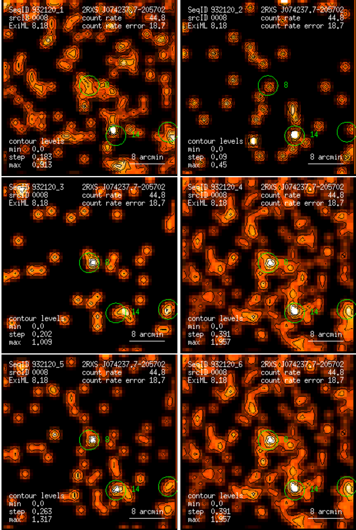
Figure 8: RASS 932120: detection 0008: band rate images, Gaussian filter: (1) PSPC channels 11 – 41, (2) 52 – 90, (3) 91 – 201, (4) 11 – 235, (5) 52 – 201, (6) 11 – 201. Broad band rates in counts/ks. Band rate contour levels in counts/ks/arcmin 2 .
