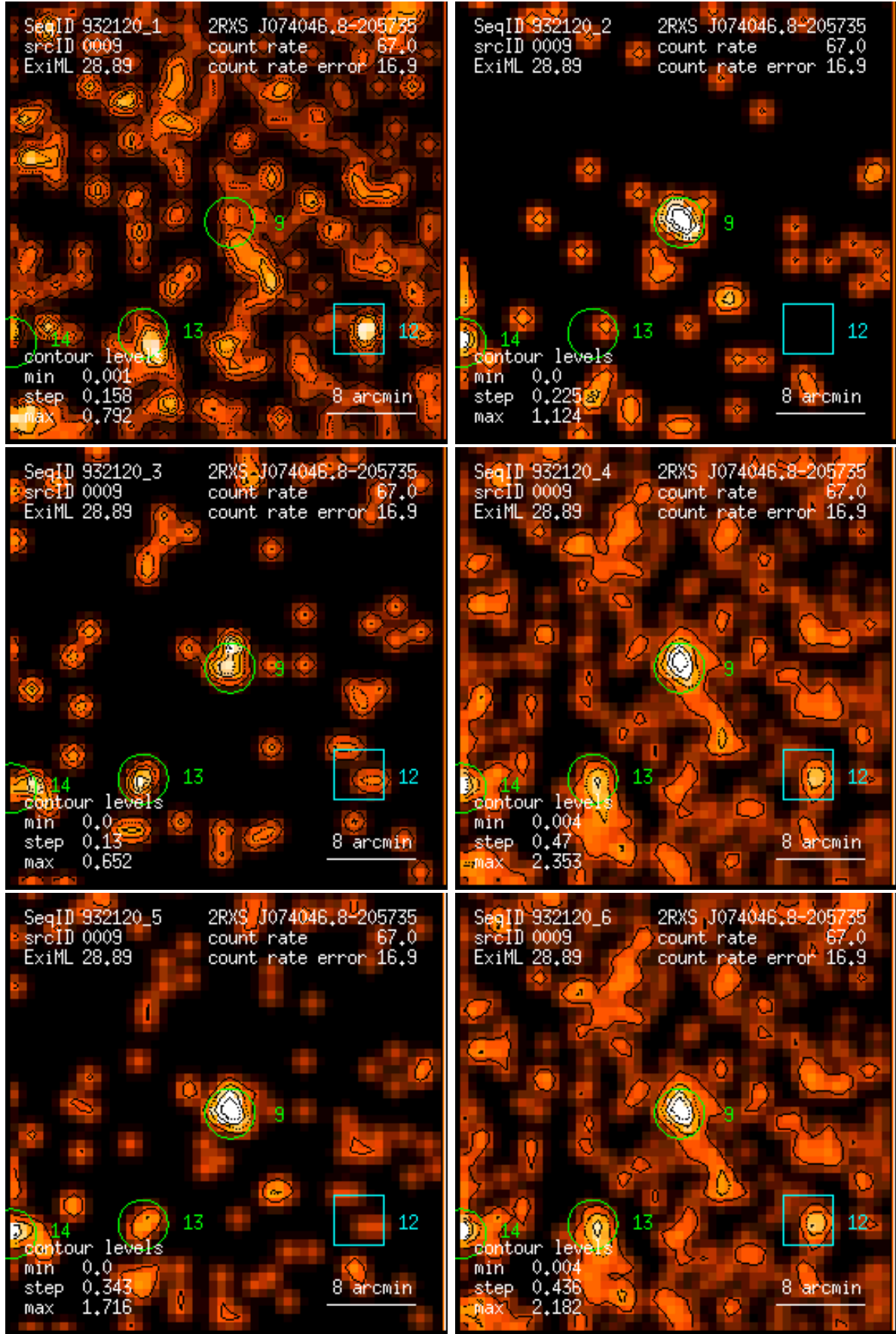
Figure 9: RASS 932120: detection 0009: band rate images, Gaussian filter: (1) PSPC channels 11 – 41, (2) 52 – 90, (3) 91 – 201, (4) 11 – 235, (5) 52 – 201, (6) 11 – 201. Broad band rates in counts/ks. Band rate contour levels in counts/ks/arcmin 2 .
