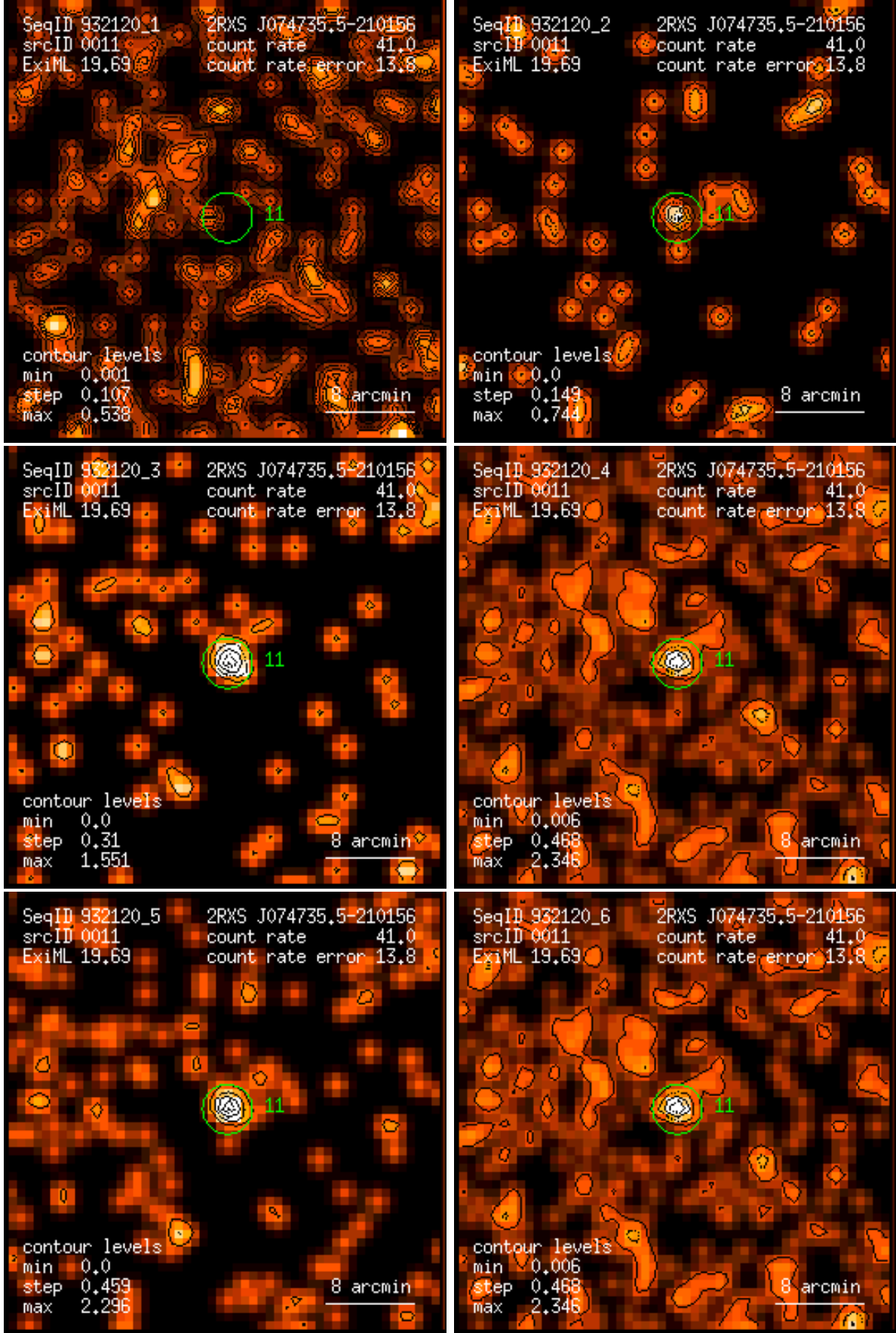
Figure 11: RASS 932120: detection 0011: band rate images, Gaussian filter: (1) PSPC channels 11 – 41, (2) 52 – 90, (3) 91 – 201, (4) 11 – 235, (5) 52 – 201, (6) 11 – 201. Broad band rates in counts/ks. Band rate contour levels in counts/ks/arcmin 2 .
