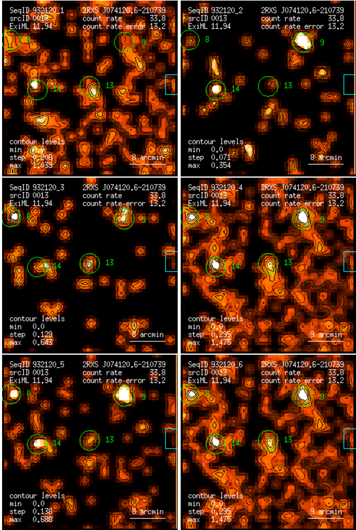
Figure 13: RASS 932120: detection 0013: band rate images, Gaussian filter: (1) PSPC channels 11 – 41, (2) 52 – 90, (3) 91 – 201, (4) 11 – 235, (5) 52 – 201, (6) 11 – 201. Broad band rates in counts/ks. Band rate contour levels in counts/ks/arcmin 2 .
