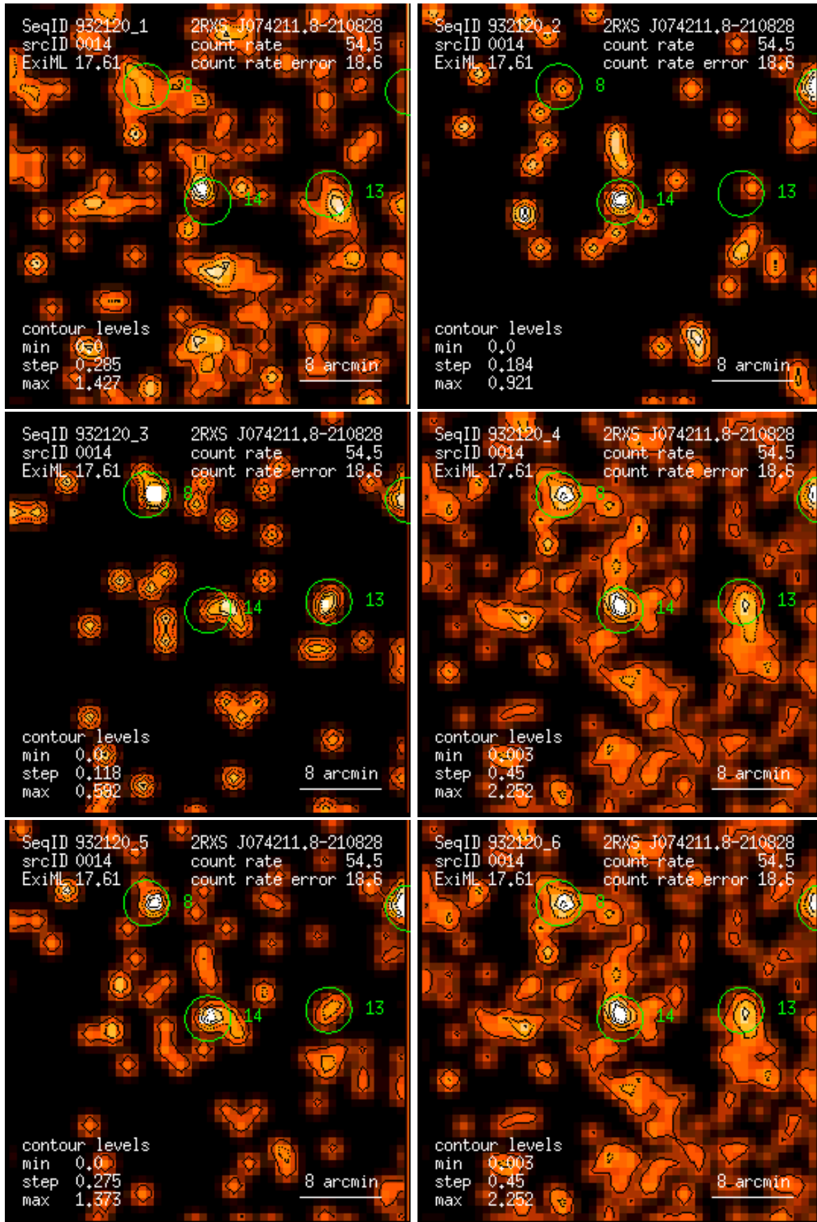
Figure 14: RASS 932120: detection 0014: band rate images, Gaussian filter: (1) PSPC channels 11 – 41, (2) 52 – 90, (3) 91 – 201, (4) 11 – 235, (5) 52 – 201, (6) 11 – 201. Broad band rates in counts/ks. Band rate contour levels in counts/ks/arcmin 2 .
