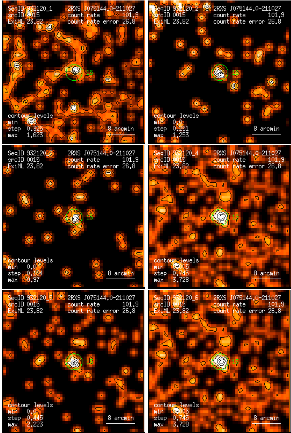
Figure 15: RASS 932120: detection 0015: band rate images, Gaussian filter: (1) PSPC channels 11 – 41, (2) 52 – 90, (3) 91 – 201, (4) 11 – 235, (5) 52 – 201, (6) 11 – 201. Broad band rates in counts/ks. Band rate contour levels in counts/ks/arcmin 2 .
