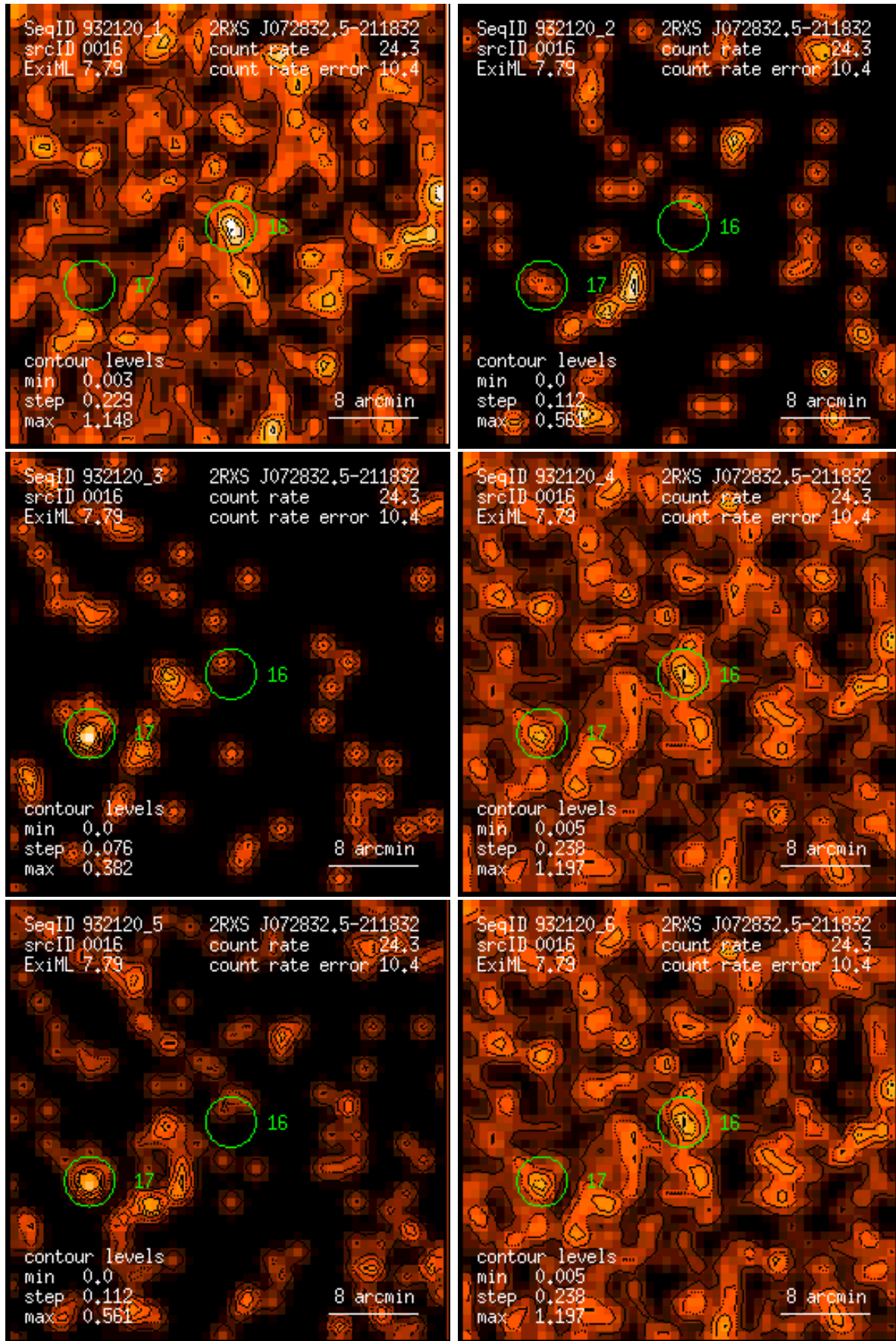
Figure 16: RASS 932120: detection 0016: band rate images, Gaussian filter: (1) PSPC channels 11 – 41, (2) 52 – 90, (3) 91 – 201, (4) 11 – 235, (5) 52 – 201, (6) 11 – 201. Broad band rates in counts/ks. Band rate contour levels in counts/ks/arcmin 2 .
