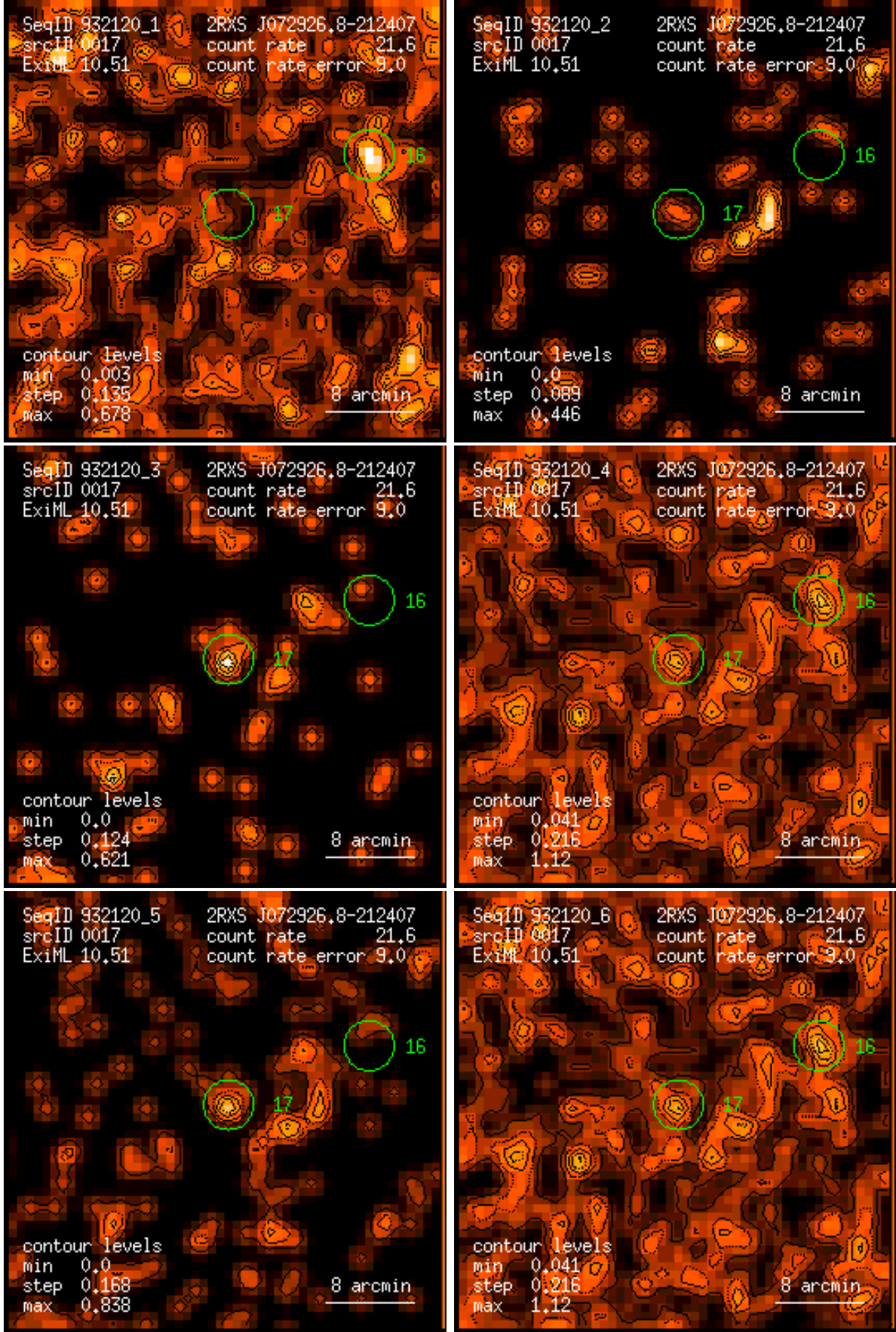
Figure 17: RASS 932120: detection 0017: band rate images, Gaussian filter: (1) PSPC channels 11 – 41, (2) 52 – 90, (3) 91 – 201, (4) 11 – 235, (5) 52 – 201, (6) 11 – 201. Broad band rates in counts/ks. Band rate contour levels in counts/ks/arcmin 2 .
