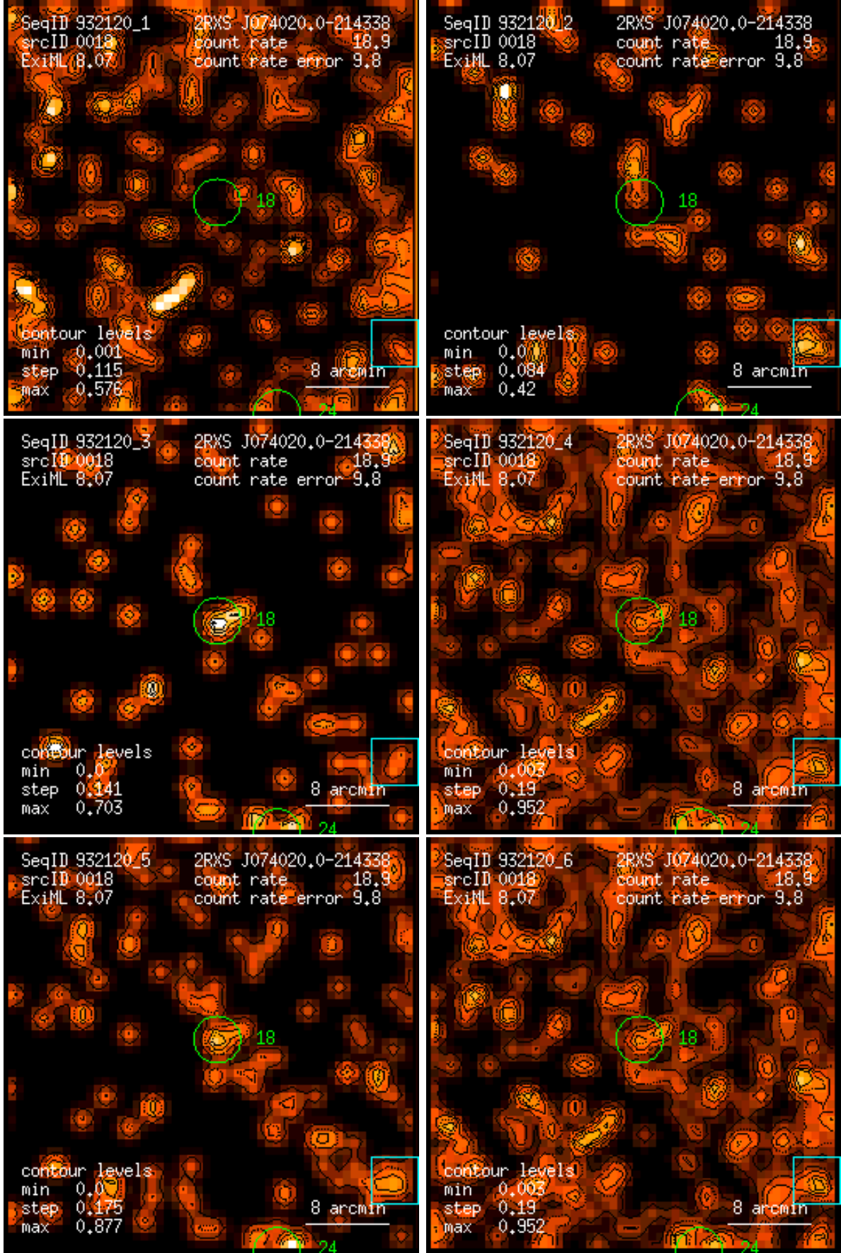
Figure 18: RASS 932120: detection 0018: band rate images, Gaussian filter: (1) PSPC channels 11 – 41, (2) 52 – 90, (3) 91 – 201, (4) 11 – 235, (5) 52 – 201, (6) 11 – 201. Broad band rates in counts/ks. Band rate contour levels in counts/ks/arcmin 2 .
