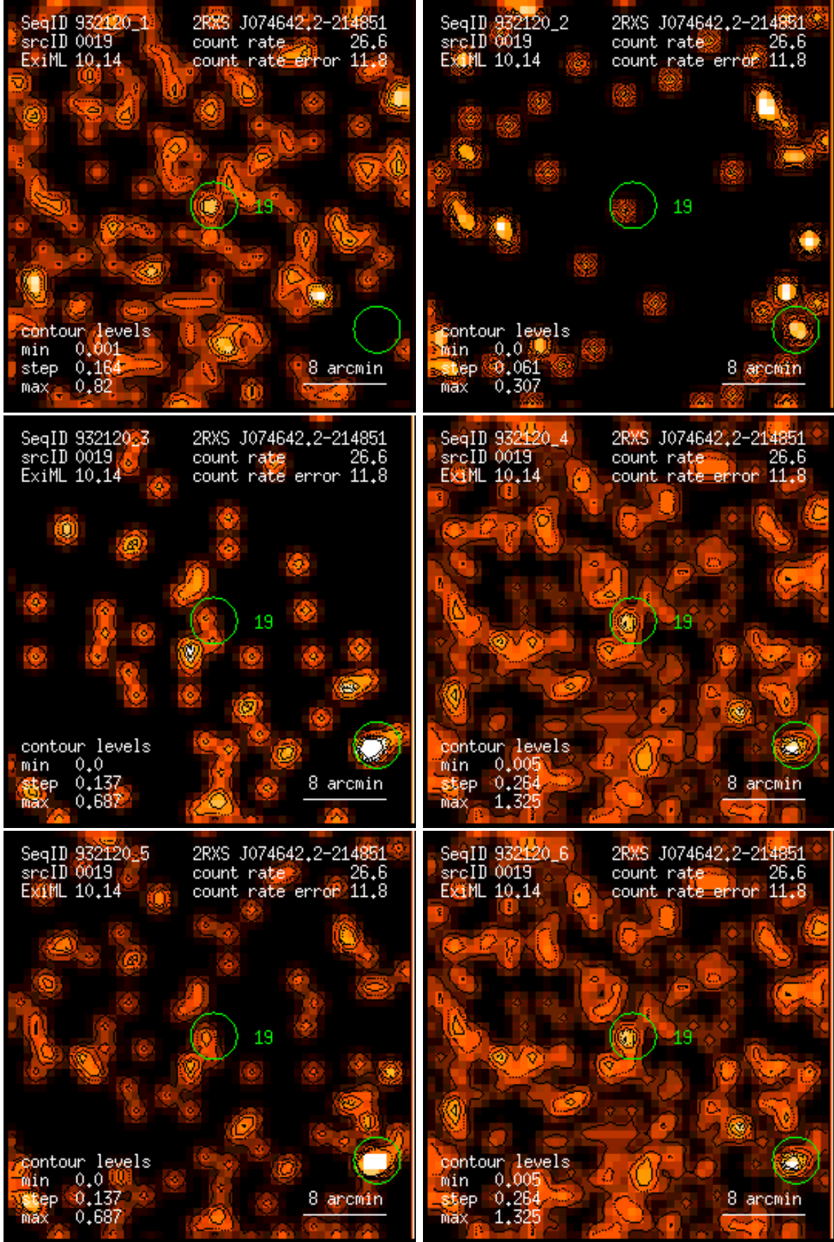
Figure 19: RASS 932120: detection 0019: band rate images, Gaussian filter: (1) PSPC channels 11 – 41, (2) 52 – 90, (3) 91 – 201, (4) 11 – 235, (5) 52 – 201, (6) 11 – 201. Broad band rates in counts/ks. Band rate contour levels in counts/ks/arcmin 2 .
