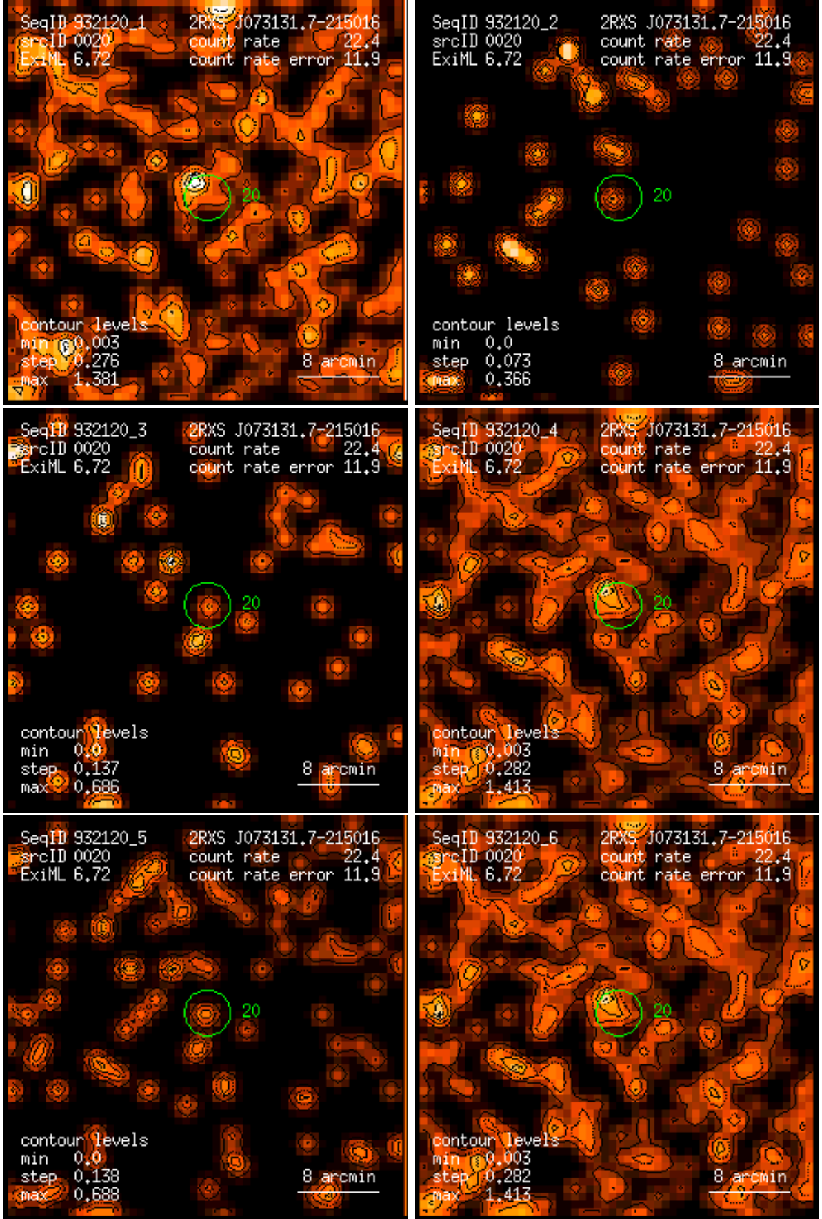
Figure 20: RASS 932120: detection 0020: band rate images, Gaussian filter: (1) PSPC channels 11 – 41, (2) 52 – 90, (3) 91 – 201, (4) 11 – 235, (5) 52 – 201, (6) 11 – 201. Broad band rates in counts/ks. Band rate contour levels in counts/ks/arcmin 2 .
