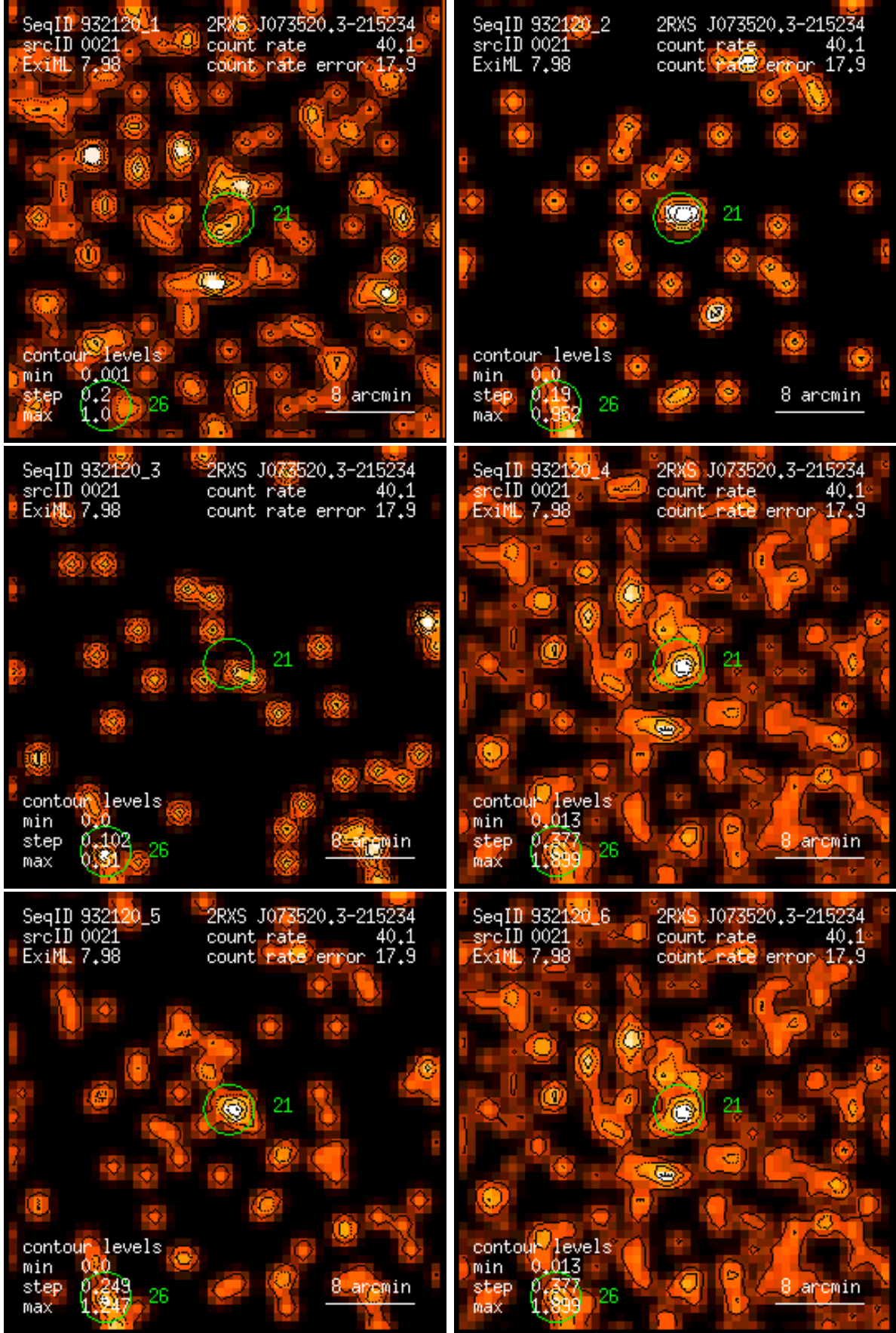
Figure 21: RASS 932120: detection 0021: band rate images, Gaussian filter: (1) PSPC channels 11 – 41, (2) 52 – 90, (3) 91 – 201, (4) 11 – 235, (5) 52 – 201, (6) 11 – 201. Broad band rates in counts/ks. Band rate contour levels in counts/ks/arcmin 2 .
