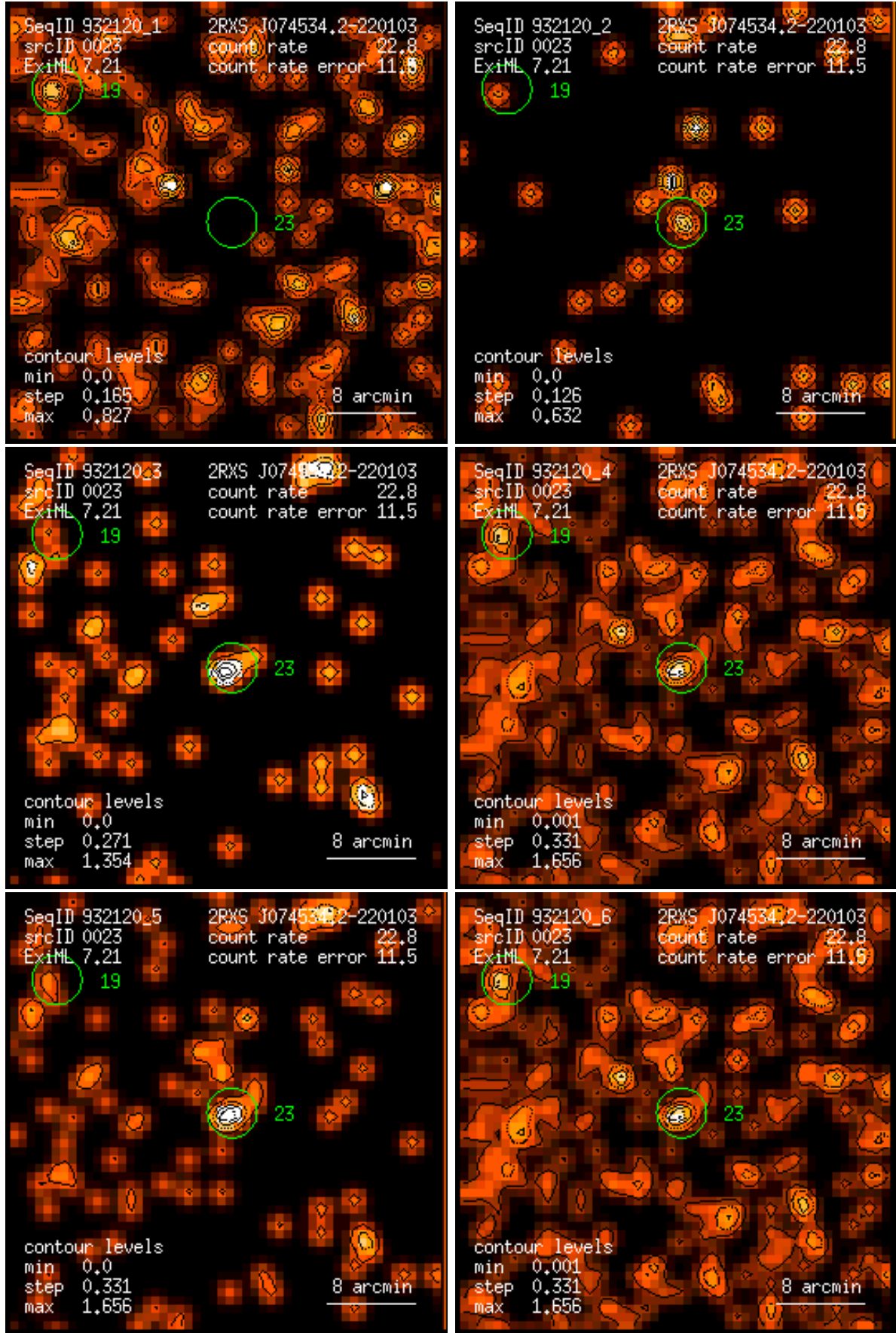
Figure 23: RASS 932120: detection 0023: band rate images, Gaussian filter: (1) PSPC channels 11 – 41, (2) 52 – 90, (3) 91 – 201, (4) 11 – 235, (5) 52 – 201, (6) 11 – 201. Broad band rates in counts/ks. Band rate contour levels in counts/ks/arcmin 2 .
