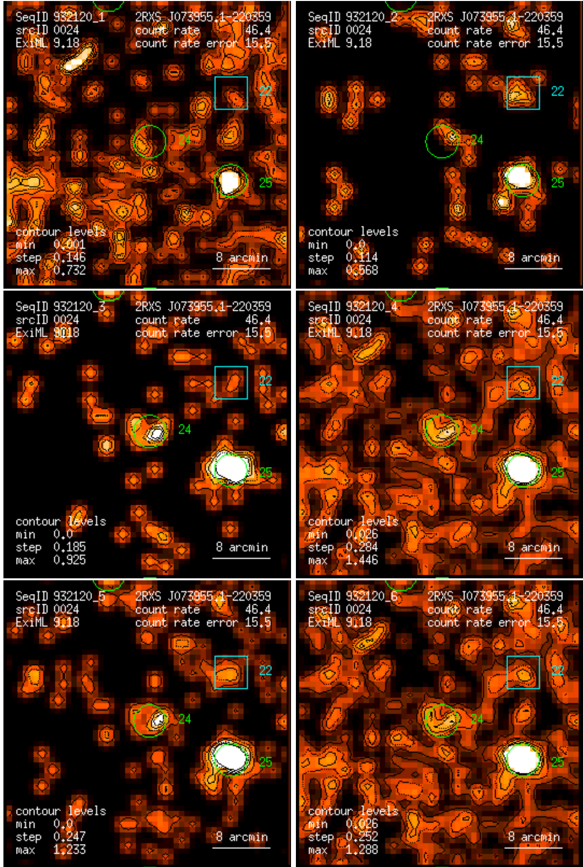
Figure 24: RASS 932120: detection 0024: band rate images, Gaussian filter: (1) PSPC channels 11 – 41, (2) 52 – 90, (3) 91 – 201, (4) 11 – 235, (5) 52 – 201, (6) 11 – 201. Broad band rates in counts/ks. Band rate contour levels in counts/ks/arcmin 2 .
