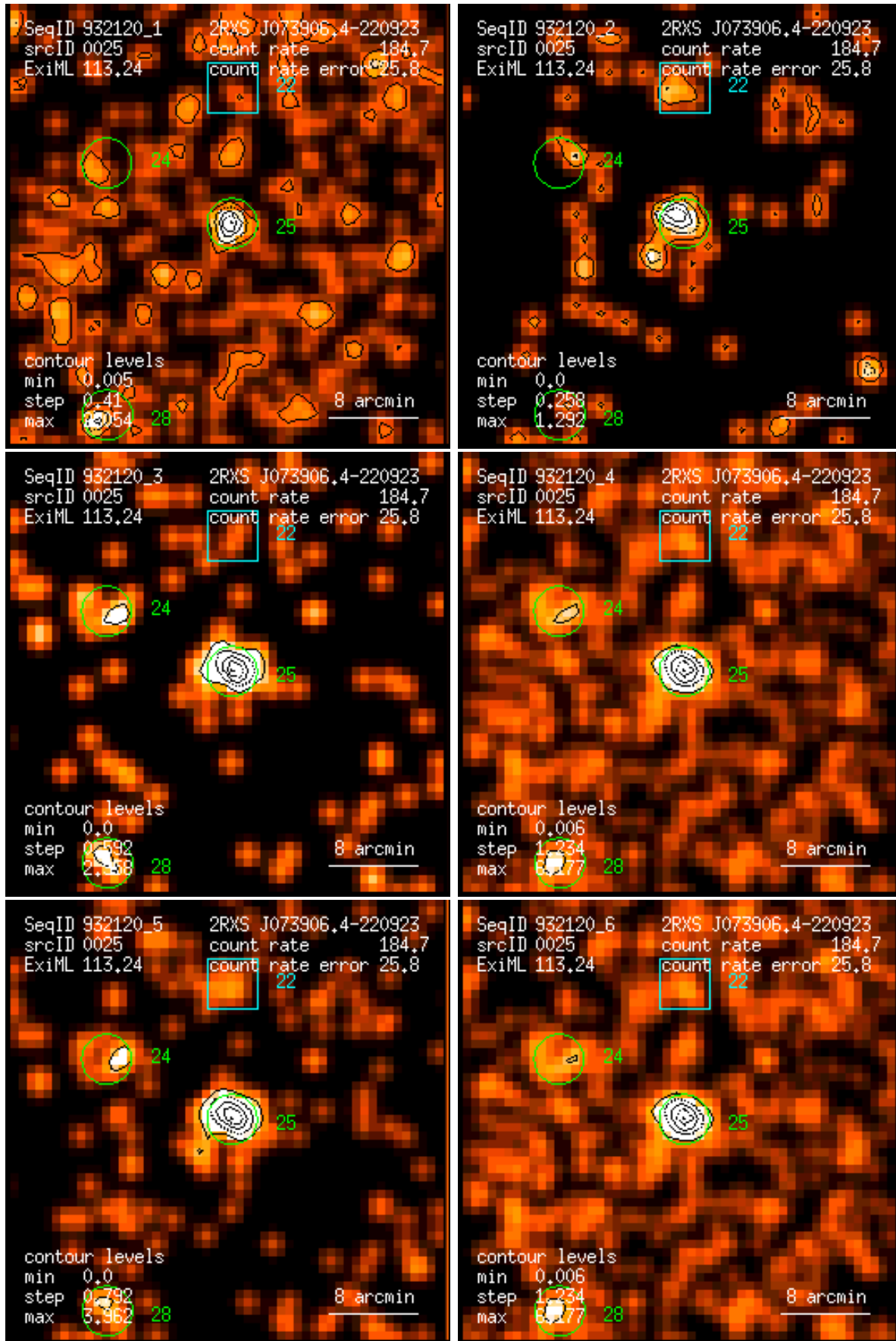
Figure 25: RASS 932120: detection 0025: band rate images, Gaussian filter: (1) PSPC channels 11 – 41, (2) 52 – 90, (3) 91 – 201, (4) 11 – 235, (5) 52 – 201, (6) 11 – 201. Broad band rates in counts/ks. Band rate contour levels in counts/ks/arcmin 2 .
