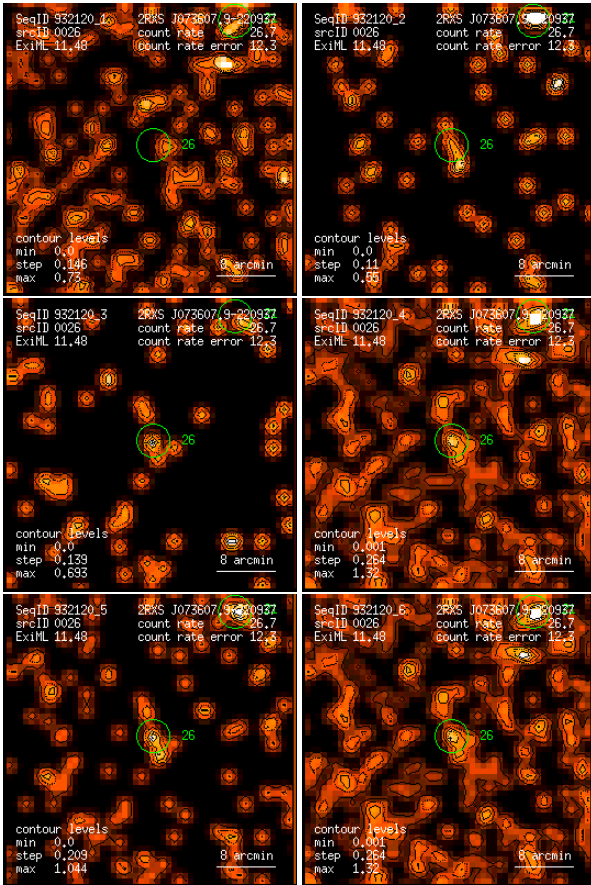
Figure 26: RASS 932120: detection 0026: band rate images, Gaussian filter: (1) PSPC channels 11 – 41, (2) 52 – 90, (3) 91 – 201, (4) 11 – 235, (5) 52 – 201, (6) 11 – 201. Broad band rates in counts/ks. Band rate contour levels in counts/ks/arcmin 2 .
