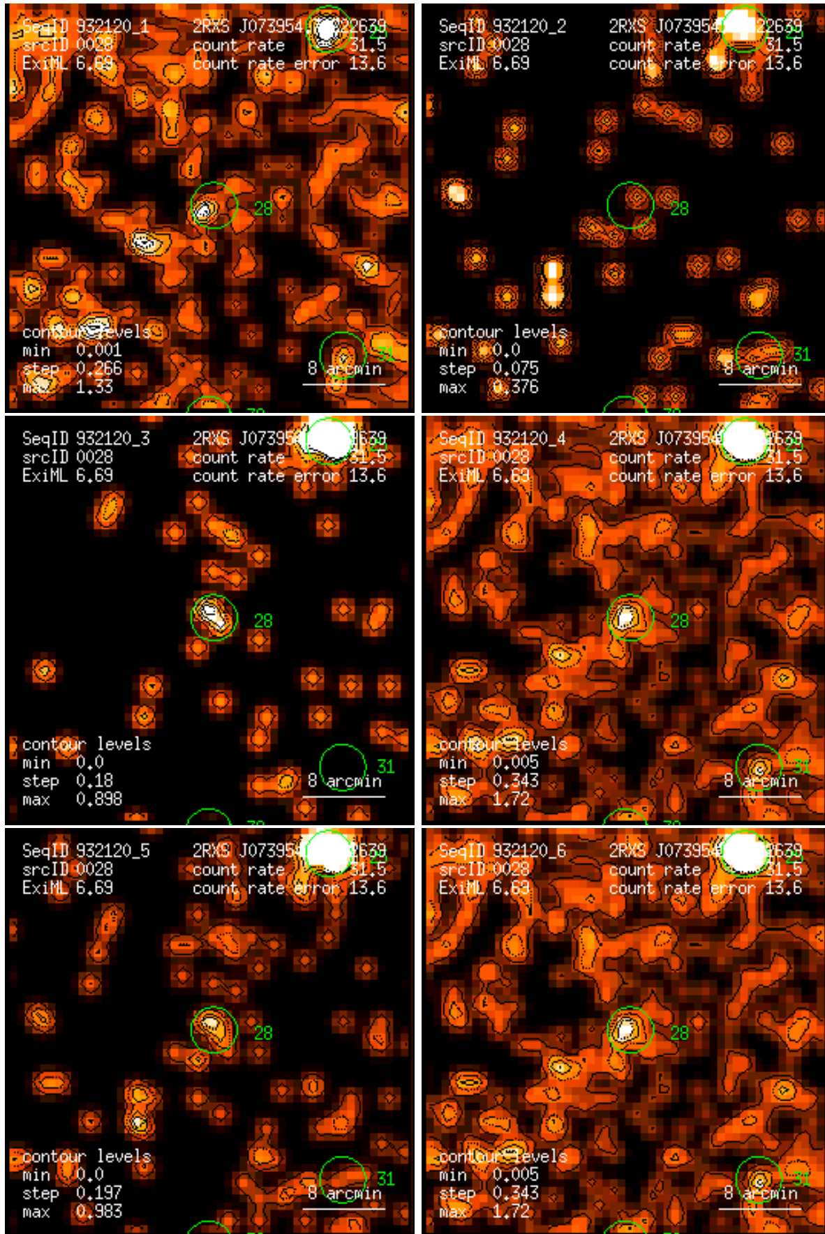
Figure 28: RASS 932120: detection 0028: band rate images, Gaussian filter: (1) PSPC channels 11 – 41, (2) 52 – 90, (3) 91 – 201, (4) 11 – 235, (5) 52 – 201, (6) 11 – 201. Broad band rates in counts/ks. Band rate contour levels in counts/ks/arcmin 2 .
