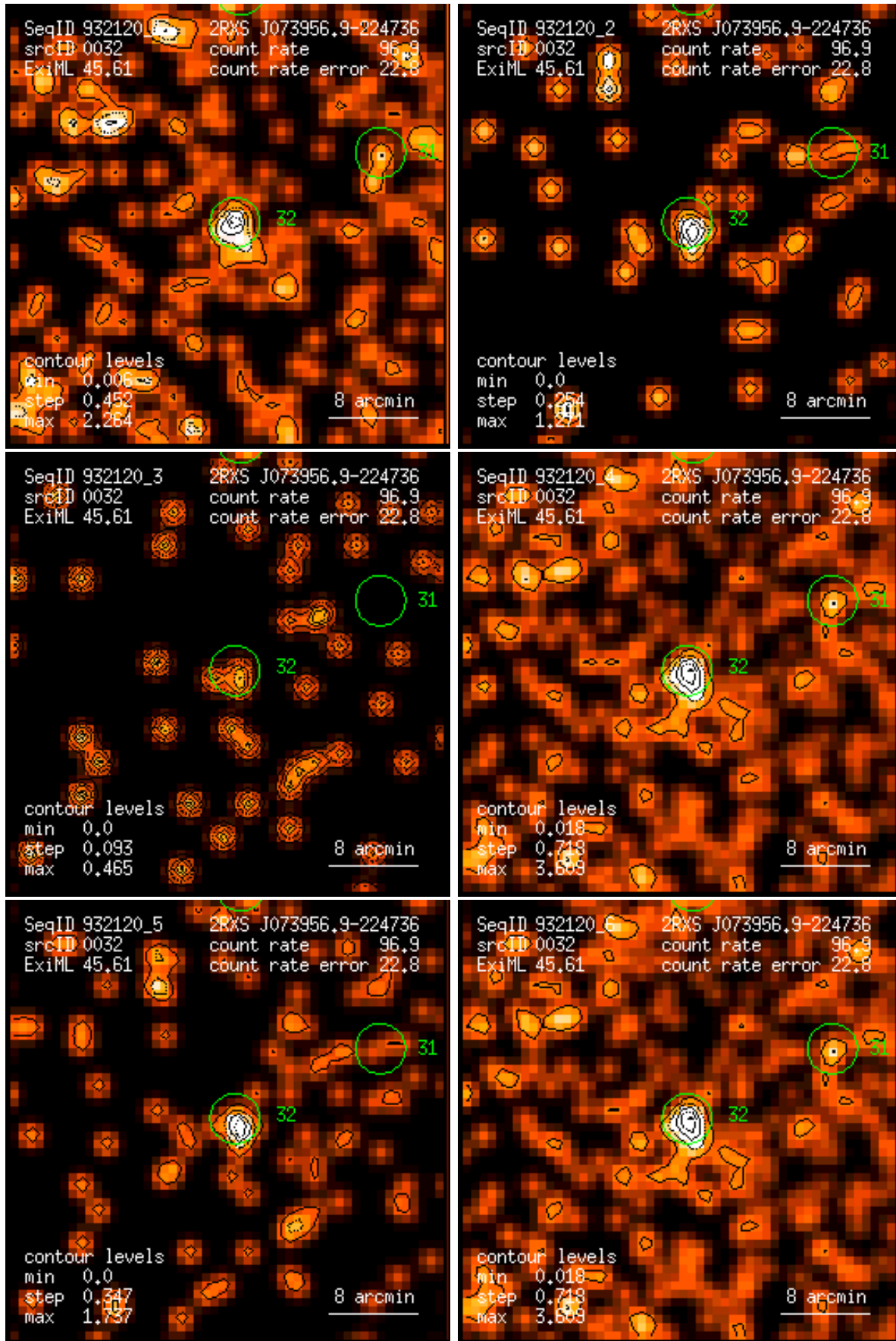
Figure 32: RASS 932120: detection 0032: band rate images, Gaussian filter: (1) PSPC channels 11 – 41, (2) 52 – 90, (3) 91 – 201, (4) 11 – 235, (5) 52 – 201, (6) 11 – 201. Broad band rates in counts/ks. Band rate contour levels in counts/ks/arcmin 2 .
