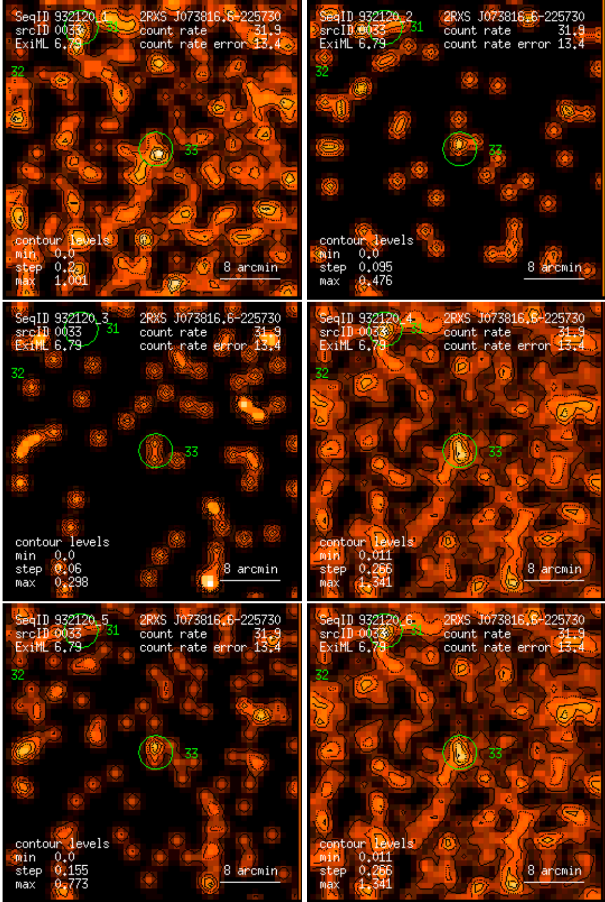
Figure 33: RASS 932120: detection 0033: band rate images, Gaussian filter: (1) PSPC channels 11 – 41, (2) 52 – 90, (3) 91 – 201, (4) 11 – 235, (5) 52 – 201, (6) 11 – 201. Broad band rates in counts/ks. Band rate contour levels in counts/ks/arcmin 2 .
