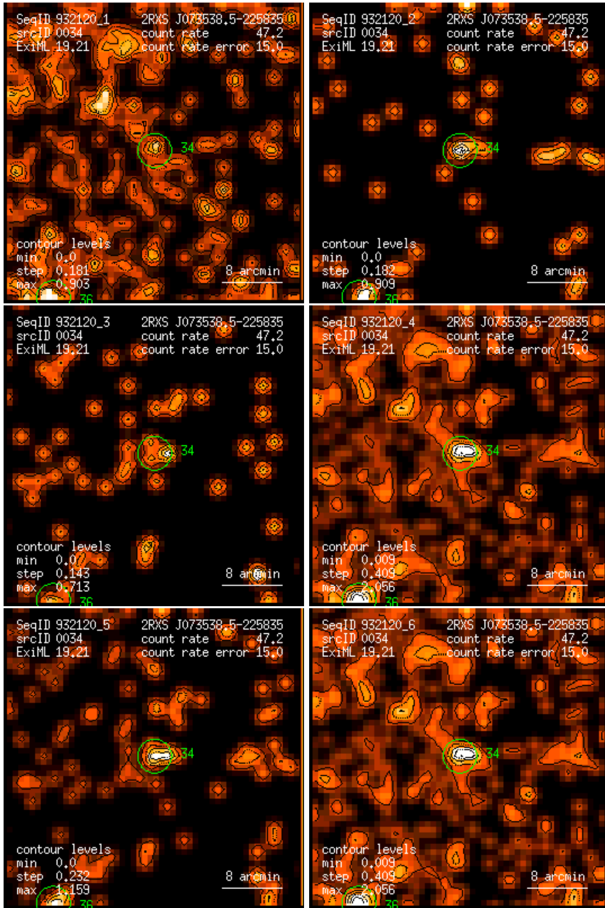
Figure 34: RASS 932120: detection 0034: band rate images, Gaussian filter: (1) PSPC channels 11 – 41, (2) 52 – 90, (3) 91 – 201, (4) 11 – 235, (5) 52 – 201, (6) 11 – 201. Broad band rates in counts/ks. Band rate contour levels in counts/ks/arcmin 2 .
