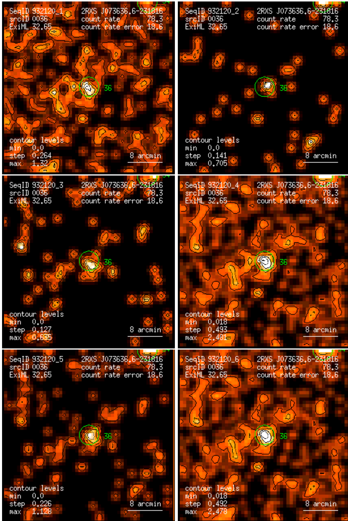
Figure 36: RASS 932120: detection 0036: band rate images, Gaussian filter: (1) PSPC channels 11 – 41, (2) 52 – 90, (3) 91 – 201, (4) 11 – 235, (5) 52 – 201, (6) 11 – 201. Broad band rates in counts/ks. Band rate contour levels in counts/ks/arcmin 2 .
