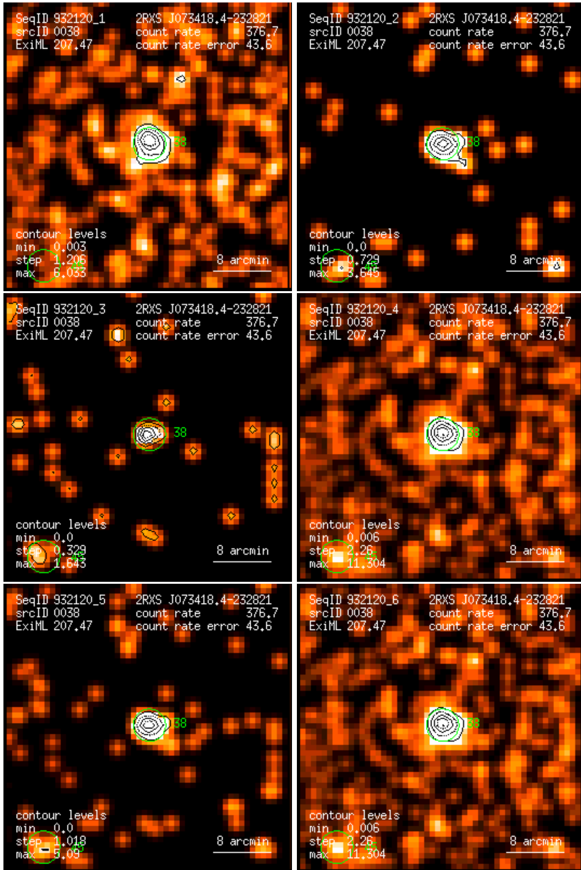
Figure 38: RASS 932120: detection 0038: band rate images, Gaussian filter: (1) PSPC channels 11 – 41, (2) 52 – 90, (3) 91 – 201, (4) 11 – 235, (5) 52 – 201, (6) 11 – 201. Broad band rates in counts/ks. Band rate contour levels in counts/ks/arcmin 2 .
